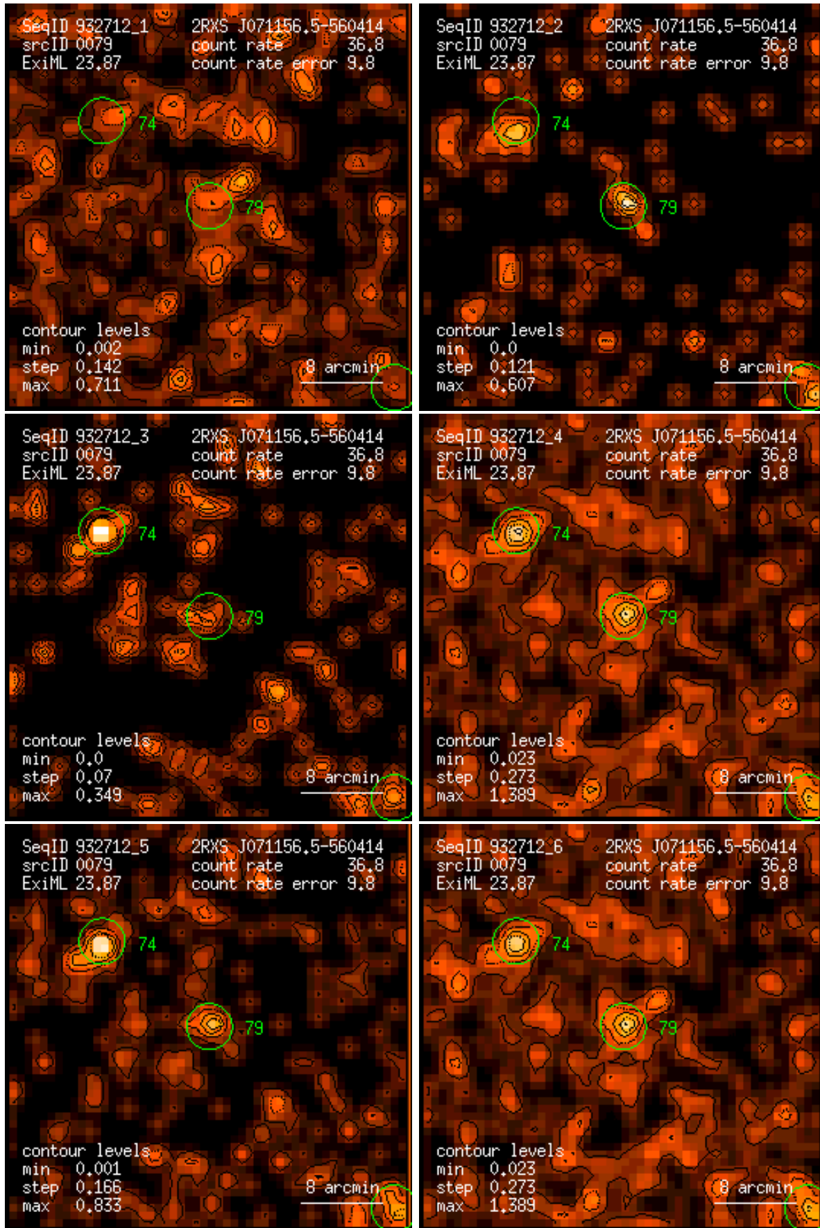
Figure 79: RASS 932712: detection 0079: band rate images, Gaussian filter: (1) PSPC channels 11 – 41, (2) 52 – 90, (3) 91 – 201, (4) 11 – 235, (5) 52 – 201, (6) 11 – 201. Broad band rates in counts/ks. Band rate contour levels in counts/ks/arcmin 2 .
