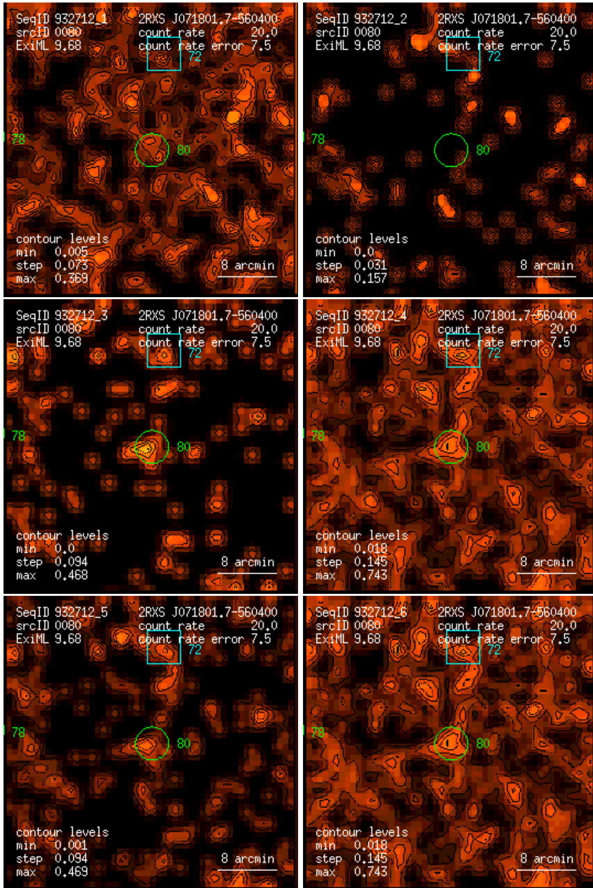
Figure 80: RASS 932712: detection 0080: band rate images, Gaussian filter: (1) PSPC channels 11 – 41, (2) 52 – 90, (3) 91 – 201, (4) 11 – 235, (5) 52 – 201, (6) 11 – 201. Broad band rates in counts/ks. Band rate contour levels in counts/ks/arcmin 2 .
