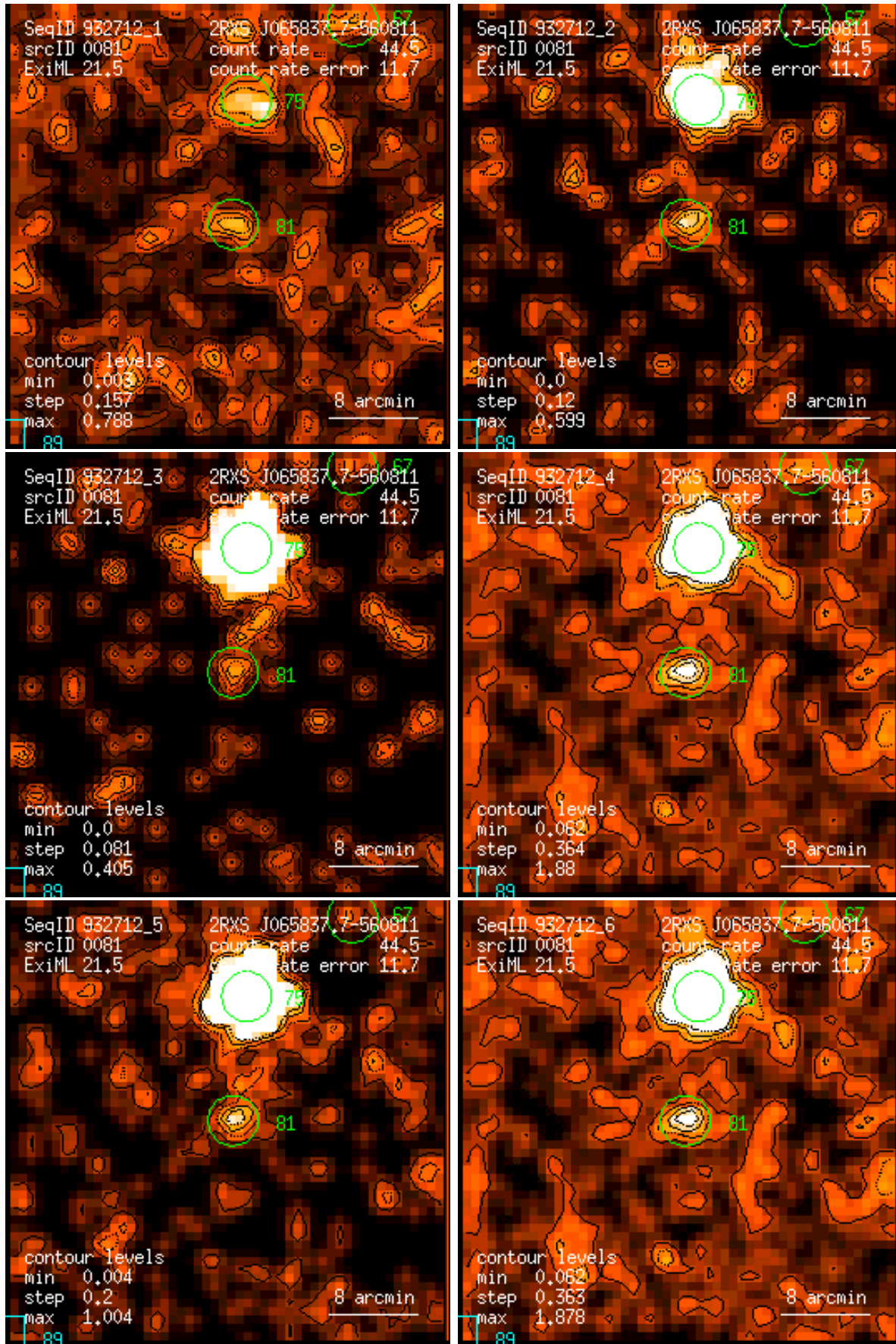
Figure 81: RASS 932712: detection 0081: band rate images, Gaussian filter: (1) PSPC channels 11 – 41, (2) 52 – 90, (3) 91 – 201, (4) 11 – 235, (5) 52 – 201, (6) 11 – 201. Broad band rates in counts/ks. Band rate contour levels in counts/ks/arcmin 2 .
