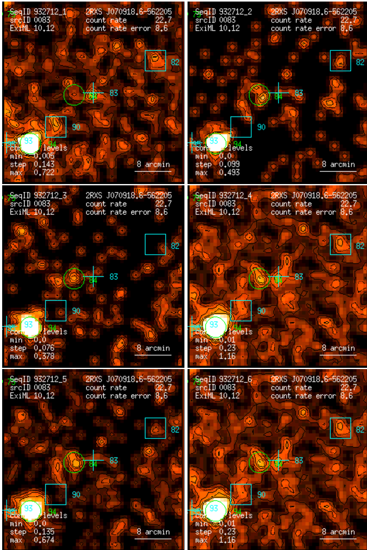
Figure 83: RASS 932712: detection 0083: band rate images, Gaussian filter: (1) PSPC channels 11 – 41, (2) 52 – 90, (3) 91 – 201, (4) 11 – 235, (5) 52 – 201, (6) 11 – 201. Broad band rates in counts/ks. Band rate contour levels in counts/ks/arcmin 2 .
