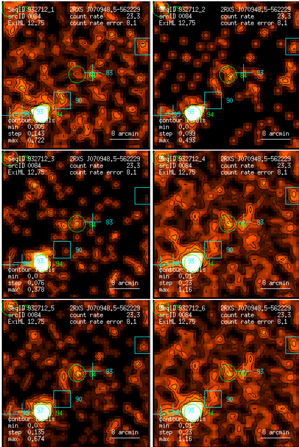
Figure 84: RASS 932712: detection 0084: band rate images, Gaussian filter: (1) PSPC channels 11 – 41, (2) 52 – 90, (3) 91 – 201, (4) 11 – 235, (5) 52 – 201, (6) 11 – 201. Broad band rates in counts/ks. Band rate contour levels in counts/ks/arcmin 2 .
