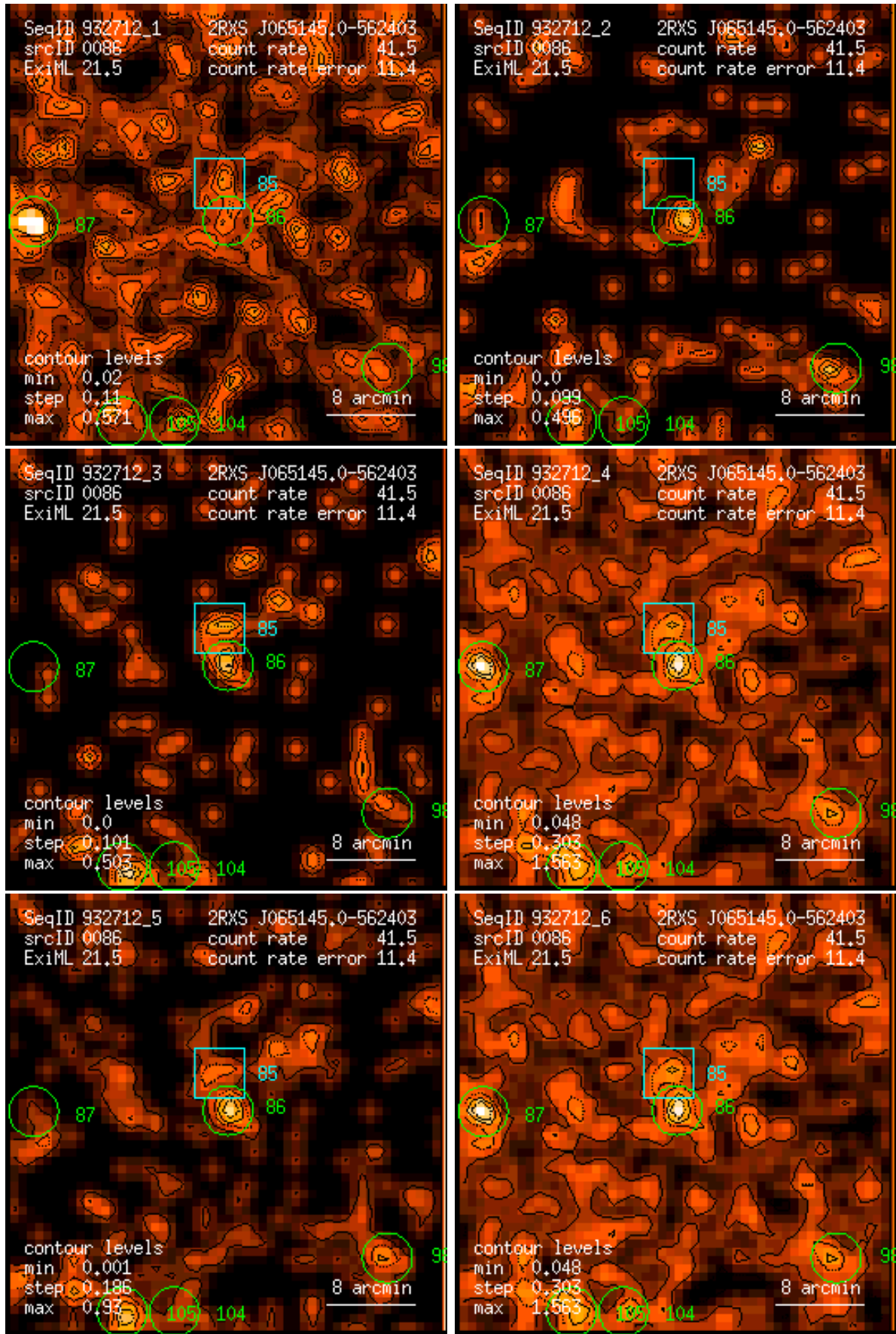
Figure 86: RASS 932712: detection 0086: band rate images, Gaussian filter: (1) PSPC channels 11 – 41, (2) 52 – 90, (3) 91 – 201, (4) 11 – 235, (5) 52 – 201, (6) 11 – 201. Broad band rates in counts/ks. Band rate contour levels in counts/ks/arcmin 2 .
