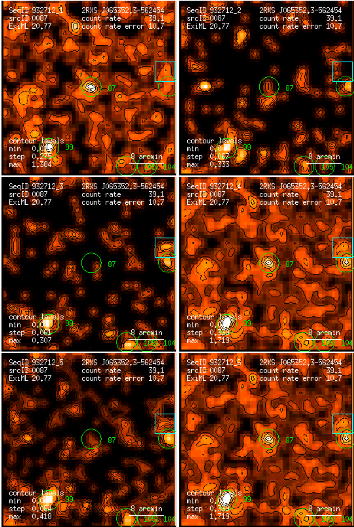
Figure 87: RASS 932712: detection 0087: band rate images, Gaussian filter: (1) PSPC channels 11 – 41, (2) 52 – 90, (3) 91 – 201, (4) 11 – 235, (5) 52 – 201, (6) 11 – 201. Broad band rates in counts/ks. Band rate contour levels in counts/ks/arcmin 2 .
