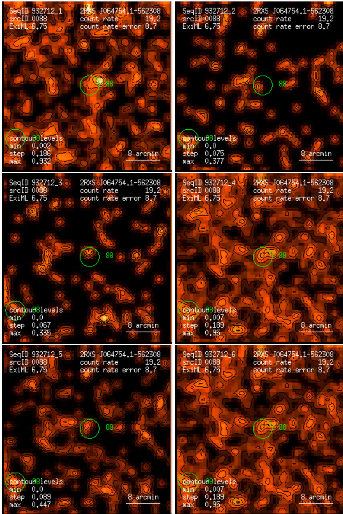
Figure 88: RASS 932712: detection 0088: band rate images, Gaussian filter: (1) PSPC channels 11 – 41, (2) 52 – 90, (3) 91 – 201, (4) 11 – 235, (5) 52 – 201, (6) 11 – 201. Broad band rates in counts/ks. Band rate contour levels in counts/ks/arcmin 2 .
