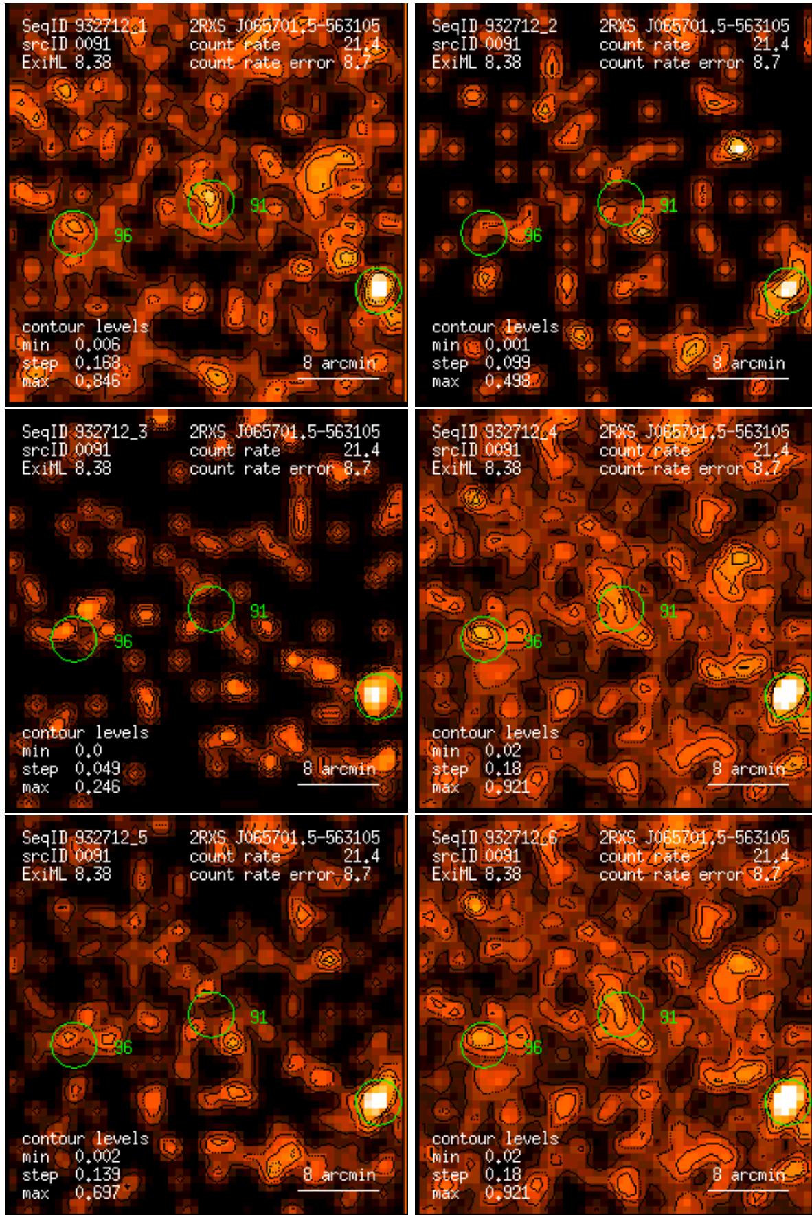
Figure 91: RASS 932712: detection 0091: band rate images, Gaussian filter: (1) PSPC channels 11 – 41, (2) 52 – 90, (3) 91 – 201, (4) 11 – 235, (5) 52 – 201, (6) 11 – 201. Broad band rates in counts/ks. Band rate contour levels in counts/ks/arcmin 2 .
