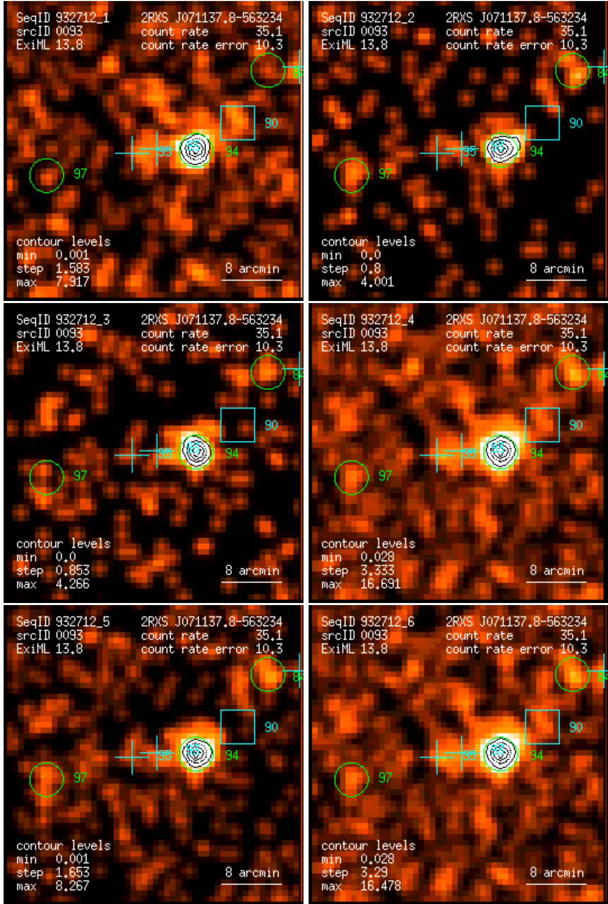
Figure 93: RASS 932712: detection 0093: band rate images, Gaussian filter: (1) PSPC channels 11 – 41, (2) 52 – 90, (3) 91 – 201, (4) 11 – 235, (5) 52 – 201, (6) 11 – 201. Broad band rates in counts/ks. Band rate contour levels in counts/ks/arcmin 2 .
