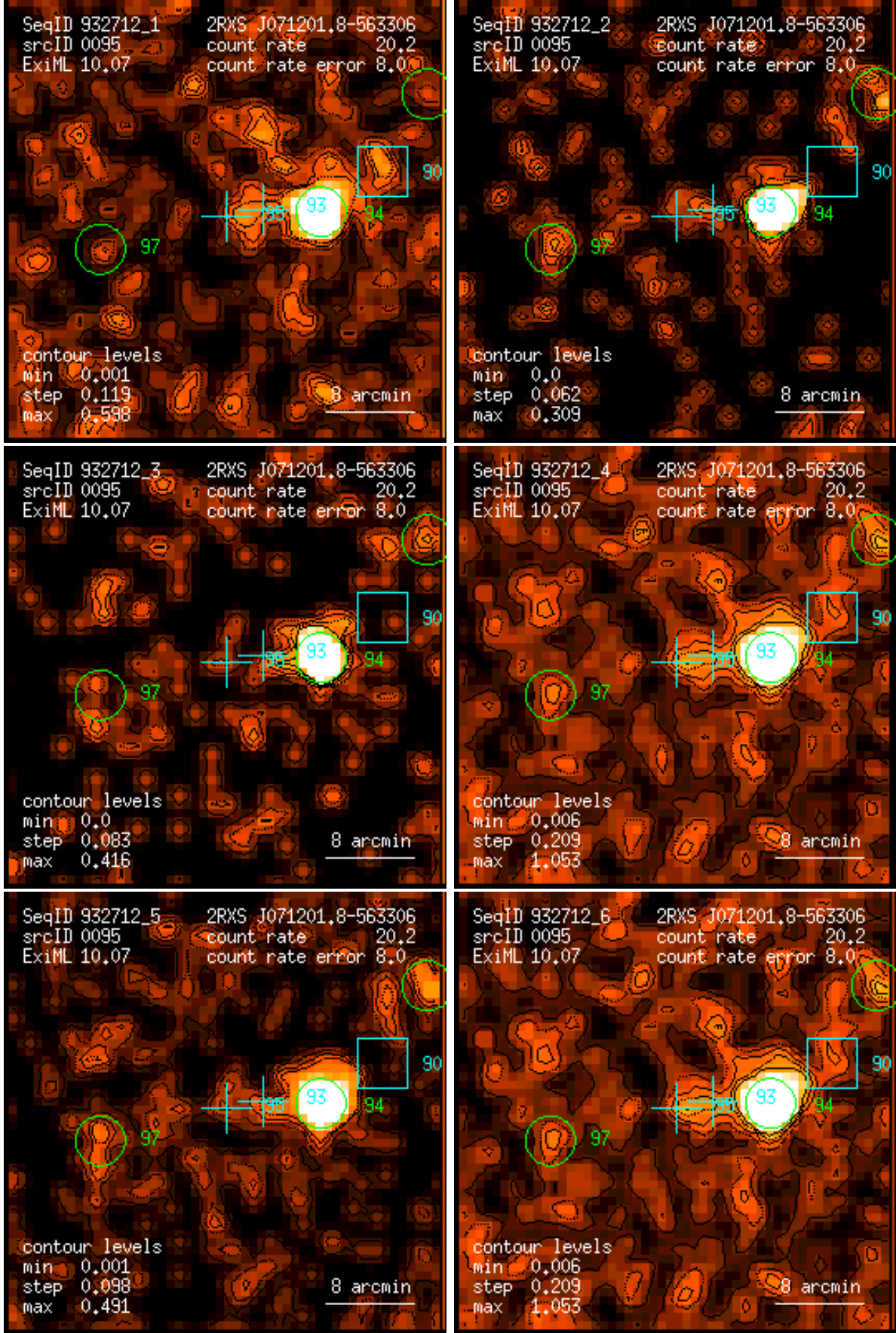
Figure 95: RASS 932712: detection 0095: band rate images, Gaussian filter: (1) PSPC channels 11 – 41, (2) 52 – 90, (3) 91 – 201, (4) 11 – 235, (5) 52 – 201, (6) 11 – 201. Broad band rates in counts/ks. Band rate contour levels in counts/ks/arcmin 2 .
