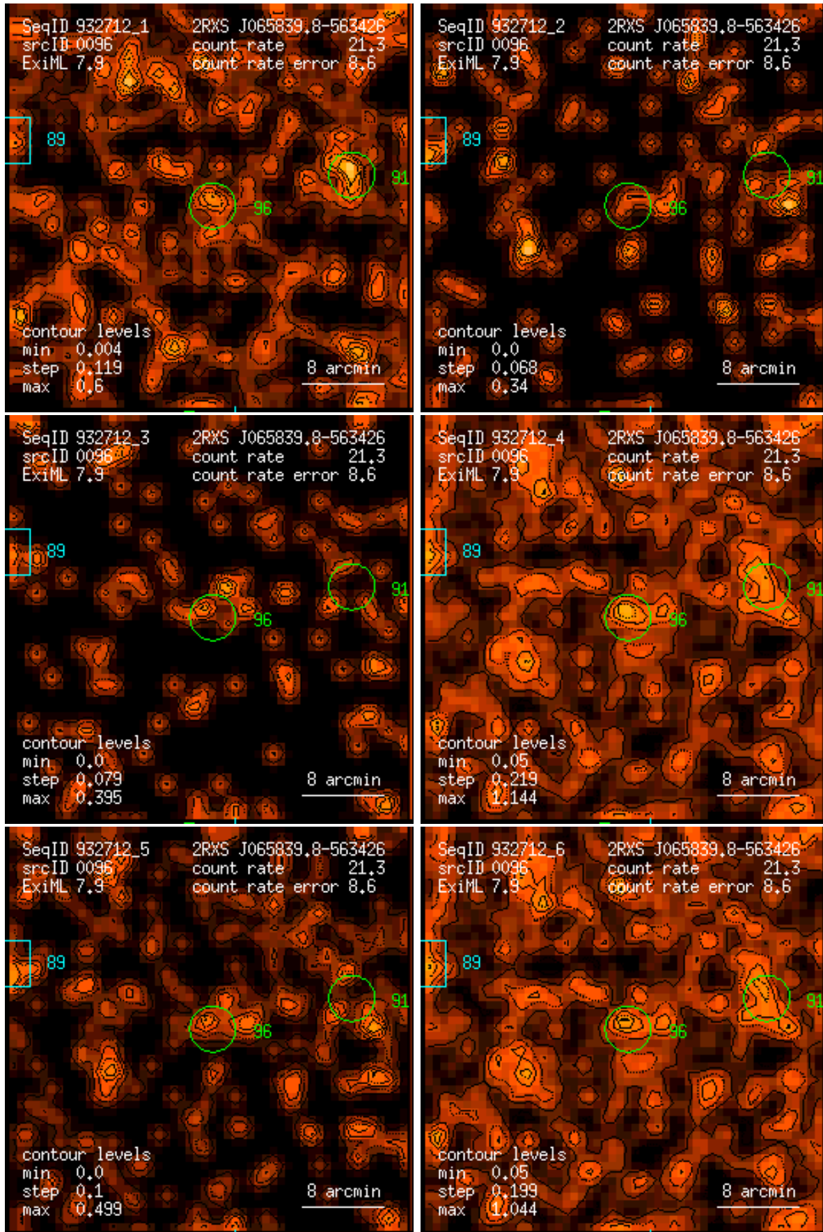
Figure 96: RASS 932712: detection 0096: band rate images, Gaussian filter: (1) PSPC channels 11 – 41, (2) 52 – 90, (3) 91 – 201, (4) 11 – 235, (5) 52 – 201, (6) 11 – 201. Broad band rates in counts/ks. Band rate contour levels in counts/ks/arcmin 2 .
