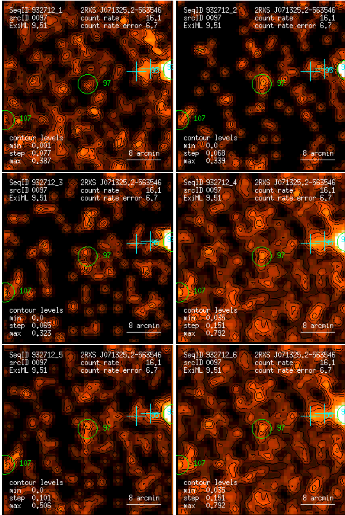
Figure 97: RASS 932712: detection 0097: band rate images, Gaussian filter: (1) PSPC channels 11 – 41, (2) 52 – 90, (3) 91 – 201, (4) 11 – 235, (5) 52 – 201, (6) 11 – 201. Broad band rates in counts/ks. Band rate contour levels in counts/ks/arcmin 2 .
