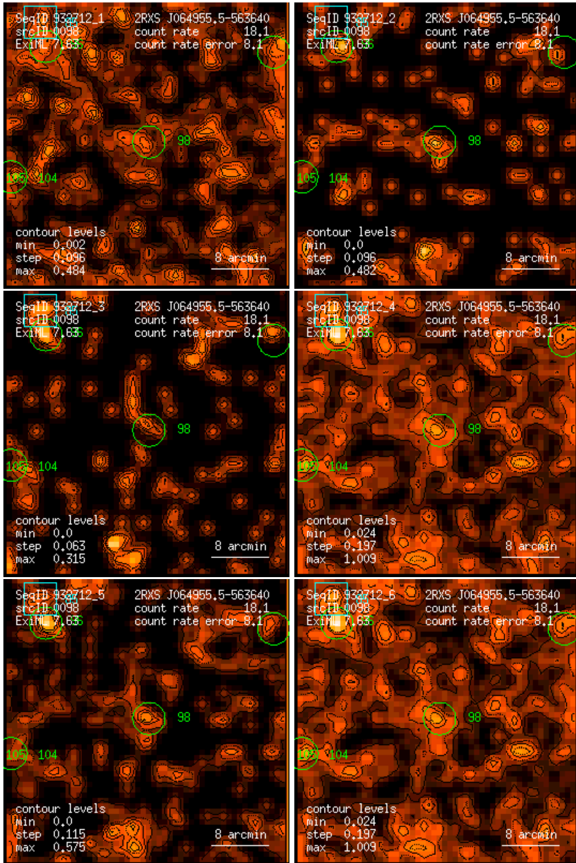
Figure 98: RASS 932712: detection 0098: band rate images, Gaussian filter: (1) PSPC channels 11 – 41, (2) 52 – 90, (3) 91 – 201, (4) 11 – 235, (5) 52 – 201, (6) 11 – 201. Broad band rates in counts/ks. Band rate contour levels in counts/ks/arcmin 2 .
