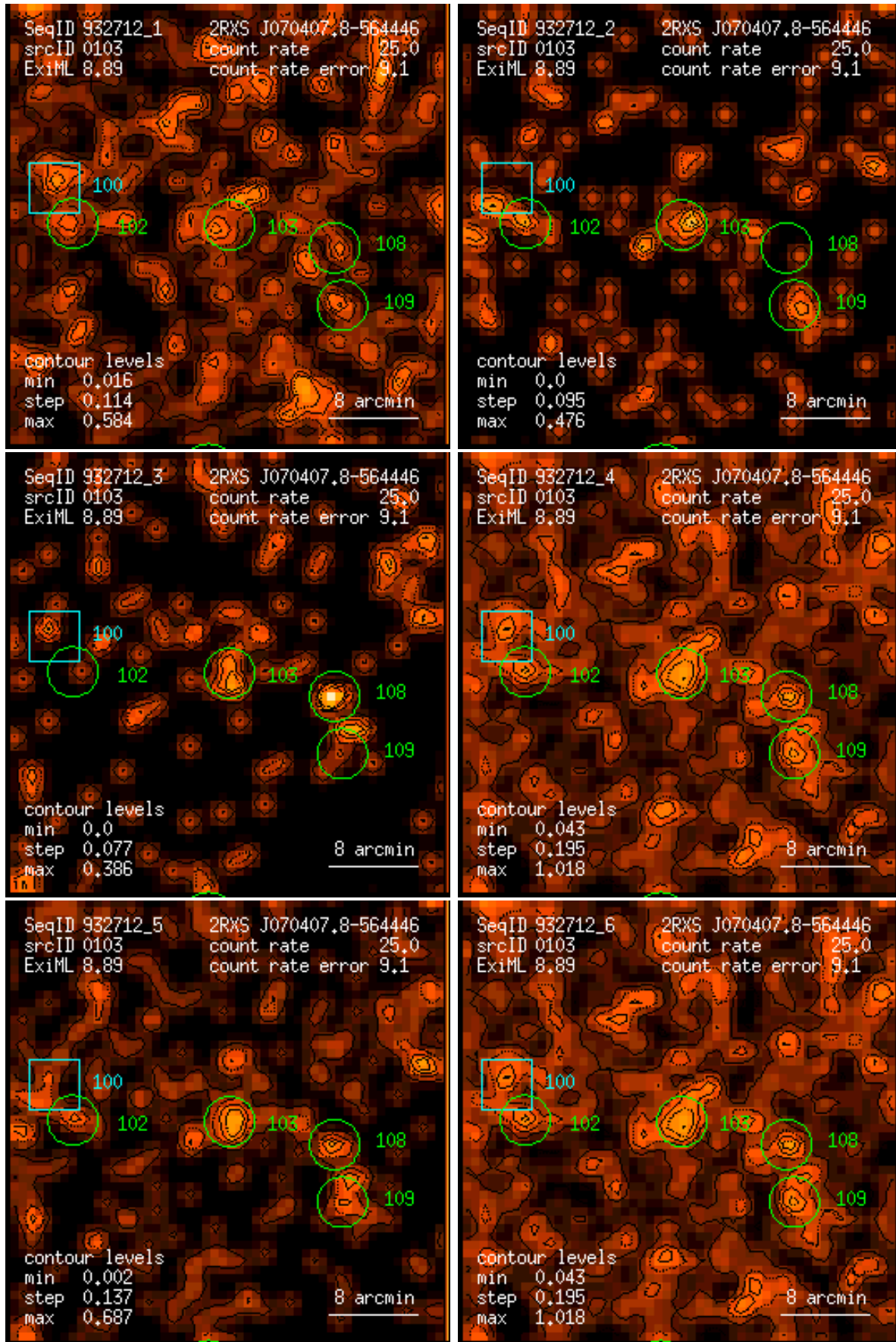
Figure 103: RASS 932712: detection 0103: band rate images, Gaussian filter: (1) PSPC channels 11 – 41, (2) 52 – 90, (3) 91 – 201, (4) 11 – 235, (5) 52 – 201, (6) 11 – 201. Broad band rates in counts/ks. Band rate contour levels in counts/ks/arcmin 2 .
