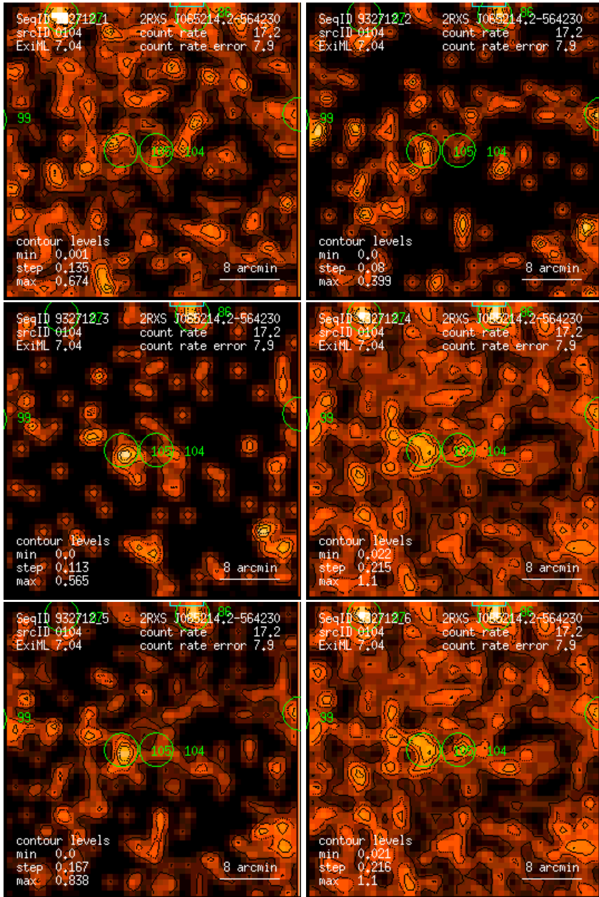
Figure 104: RASS 932712: detection 0104: band rate images, Gaussian filter: (1) PSPC channels 11 – 41, (2) 52 – 90, (3) 91 – 201, (4) 11 – 235, (5) 52 – 201, (6) 11 – 201. Broad band rates in counts/ks. Band rate contour levels in counts/ks/arcmin 2 .
