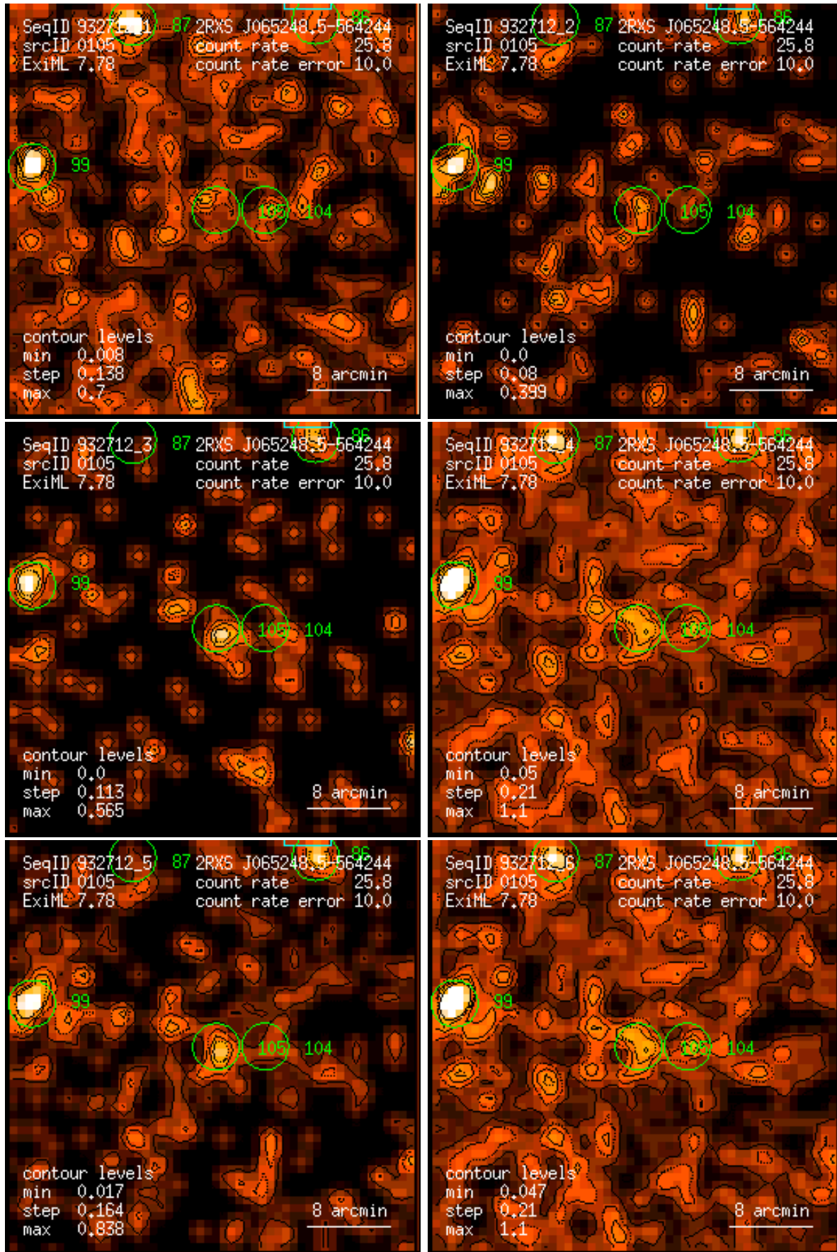
Figure 105: RASS 932712: detection 0105: band rate images, Gaussian filter: (1) PSPC channels 11 – 41, (2) 52 – 90, (3) 91 – 201, (4) 11 – 235, (5) 52 – 201, (6) 11 – 201. Broad band rates in counts/ks. Band rate contour levels in counts/ks/arcmin 2 .
