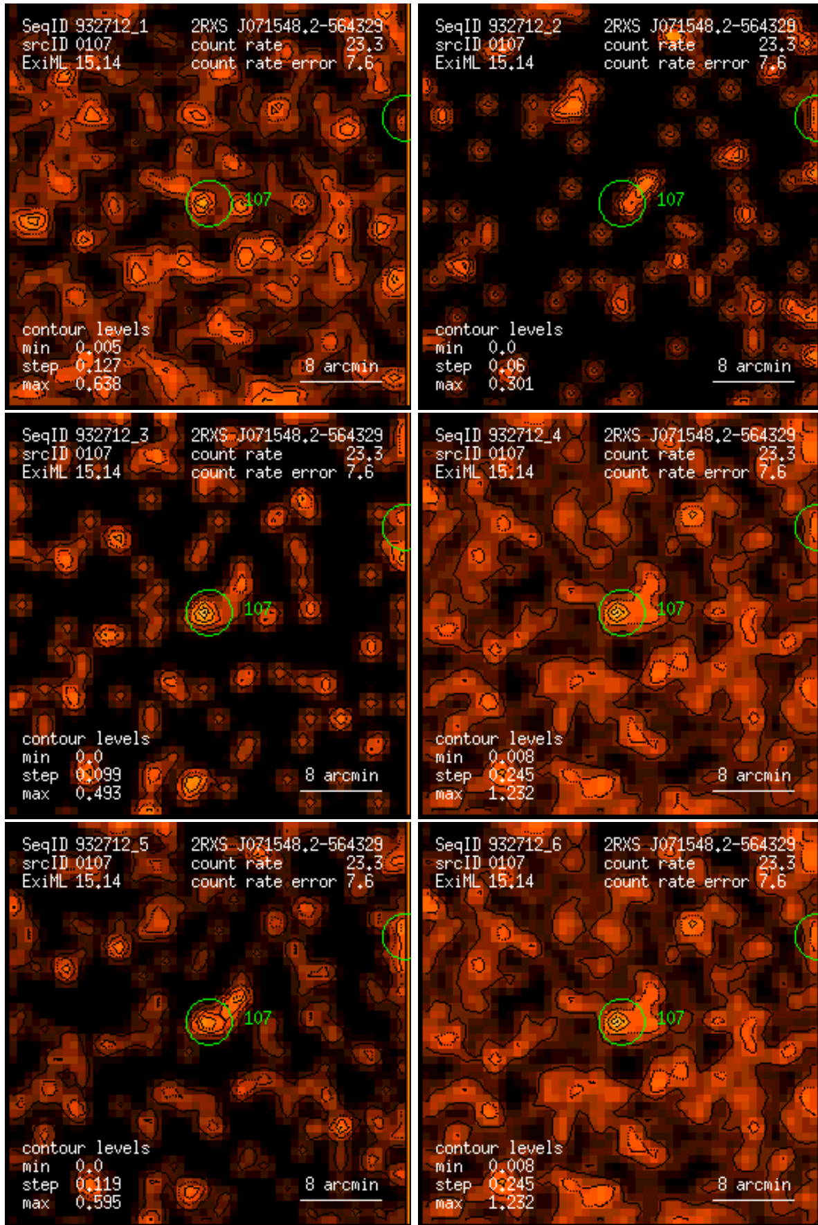
Figure 107: RASS 932712: detection 0107: band rate images, Gaussian filter: (1) PSPC channels 11 – 41, (2) 52 – 90, (3) 91 – 201, (4) 11 – 235, (5) 52 – 201, (6) 11 – 201. Broad band rates in counts/ks. Band rate contour levels in counts/ks/arcmin 2 .
