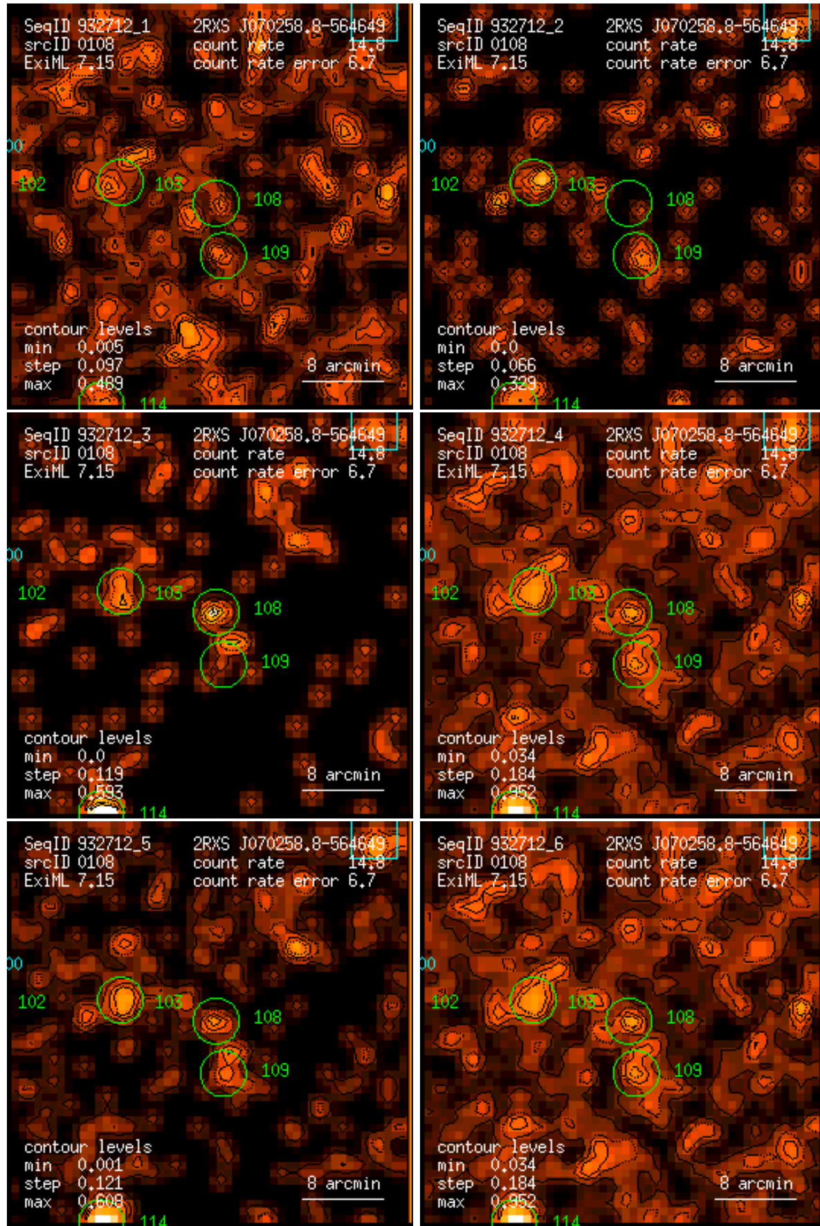
Figure 108: RASS 932712: detection 0108: band rate images, Gaussian filter: (1) PSPC channels 11 – 41, (2) 52 – 90, (3) 91 – 201, (4) 11 – 235, (5) 52 – 201, (6) 11 – 201. Broad band rates in counts/ks. Band rate contour levels in counts/ks/arcmin 2 .
