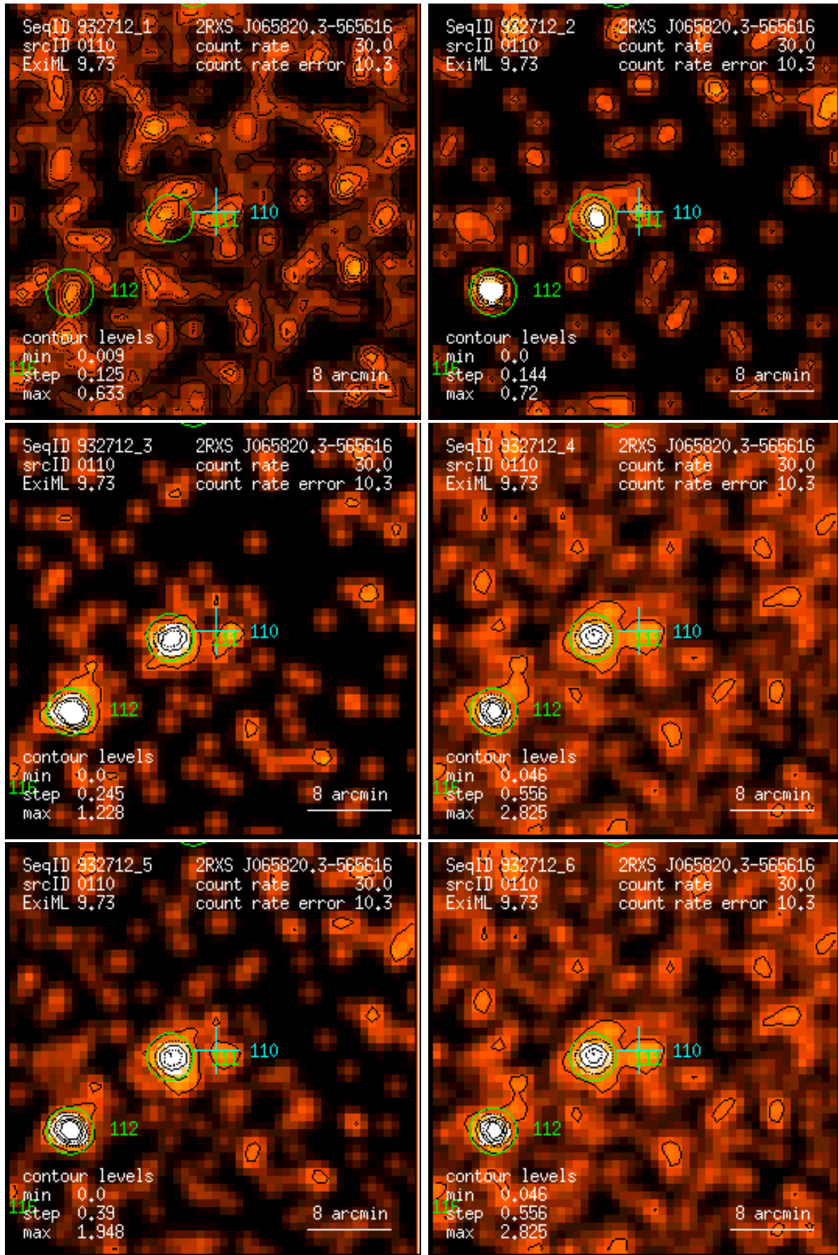
Figure 110: RASS 932712: detection 0110: band rate images, Gaussian filter: (1) PSPC channels 11 – 41, (2) 52 – 90, (3) 91 – 201, (4) 11 – 235, (5) 52 – 201, (6) 11 – 201. Broad band rates in counts/ks. Band rate contour levels in counts/ks/arcmin 2 .
