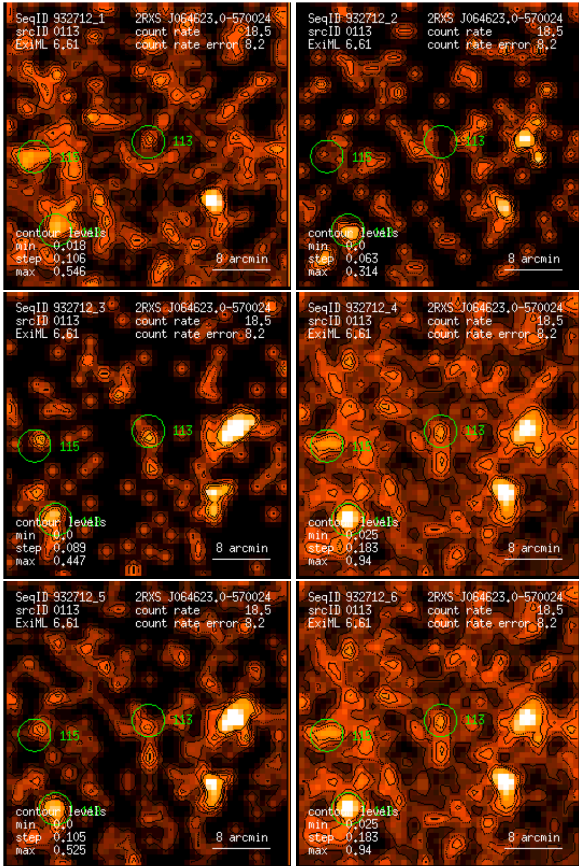
Figure 113: RASS 932712: detection 0113: band rate images, Gaussian filter: (1) PSPC channels 11 – 41, (2) 52 – 90, (3) 91 – 201, (4) 11 – 235, (5) 52 – 201, (6) 11 – 201. Broad band rates in counts/ks. Band rate contour levels in counts/ks/arcmin 2 .
