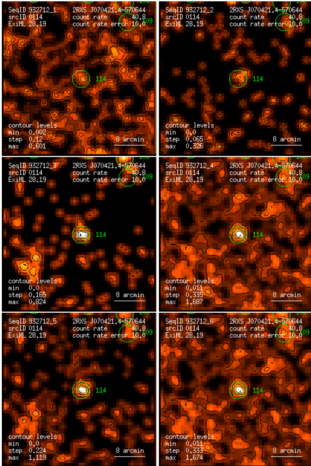
Figure 114: RASS 932712: detection 0114: band rate images, Gaussian filter: (1) PSPC channels 11 – 41, (2) 52 – 90, (3) 91 – 201, (4) 11 – 235, (5) 52 – 201, (6) 11 – 201. Broad band rates in counts/ks. Band rate contour levels in counts/ks/arcmin 2 .
