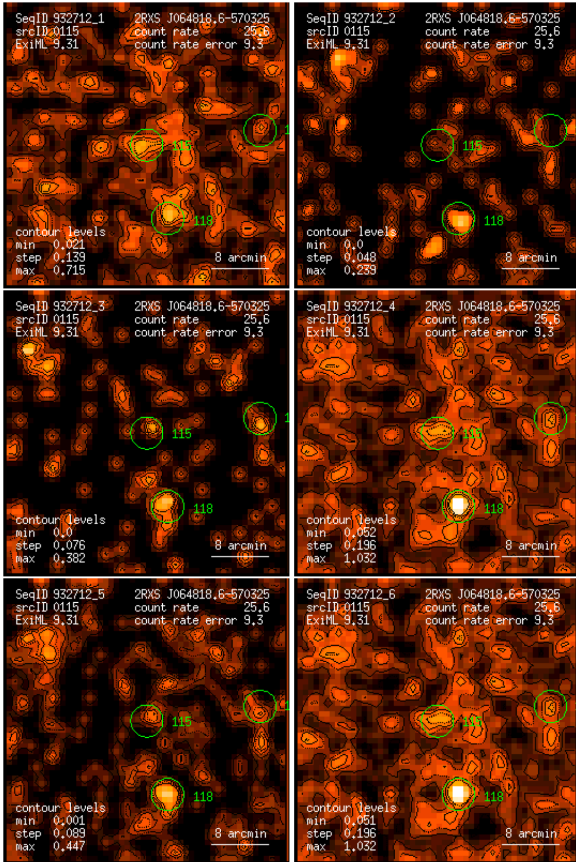
Figure 115: RASS 932712: detection 0115: band rate images, Gaussian filter: (1) PSPC channels 11 – 41, (2) 52 – 90, (3) 91 – 201, (4) 11 – 235, (5) 52 – 201, (6) 11 – 201. Broad band rates in counts/ks. Band rate contour levels in counts/ks/arcmin 2 .
