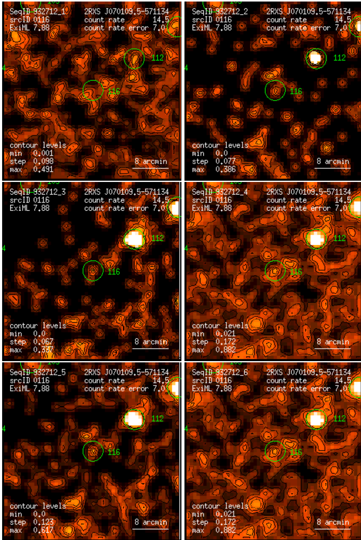
Figure 116: RASS 932712: detection 0116: band rate images, Gaussian filter: (1) PSPC channels 11 – 41, (2) 52 – 90, (3) 91 – 201, (4) 11 – 235, (5) 52 – 201, (6) 11 – 201. Broad band rates in counts/ks. Band rate contour levels in counts/ks/arcmin 2 .
