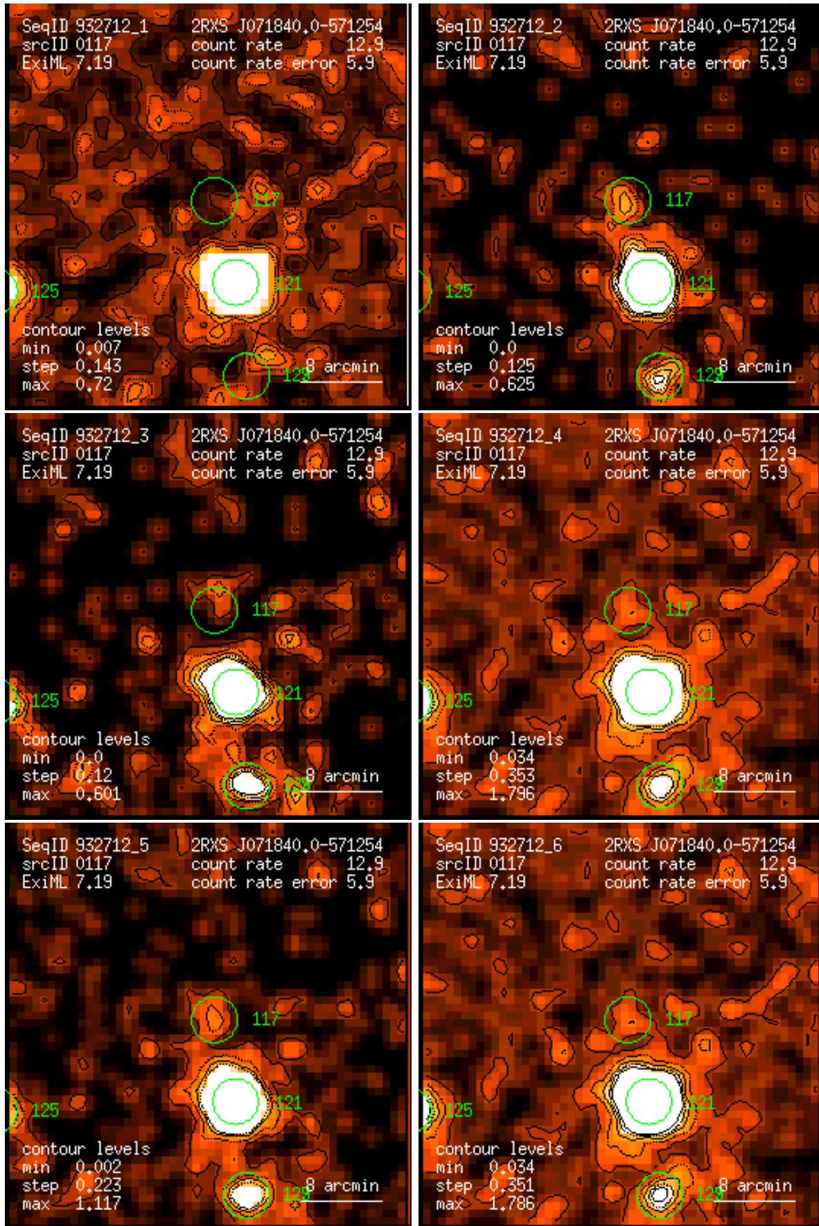
Figure 117: RASS 932712: detection 0117: band rate images, Gaussian filter: (1) PSPC channels 11 – 41, (2) 52 – 90, (3) 91 – 201, (4) 11 – 235, (5) 52 – 201, (6) 11 – 201. Broad band rates in counts/ks. Band rate contour levels in counts/ks/arcmin 2 .
