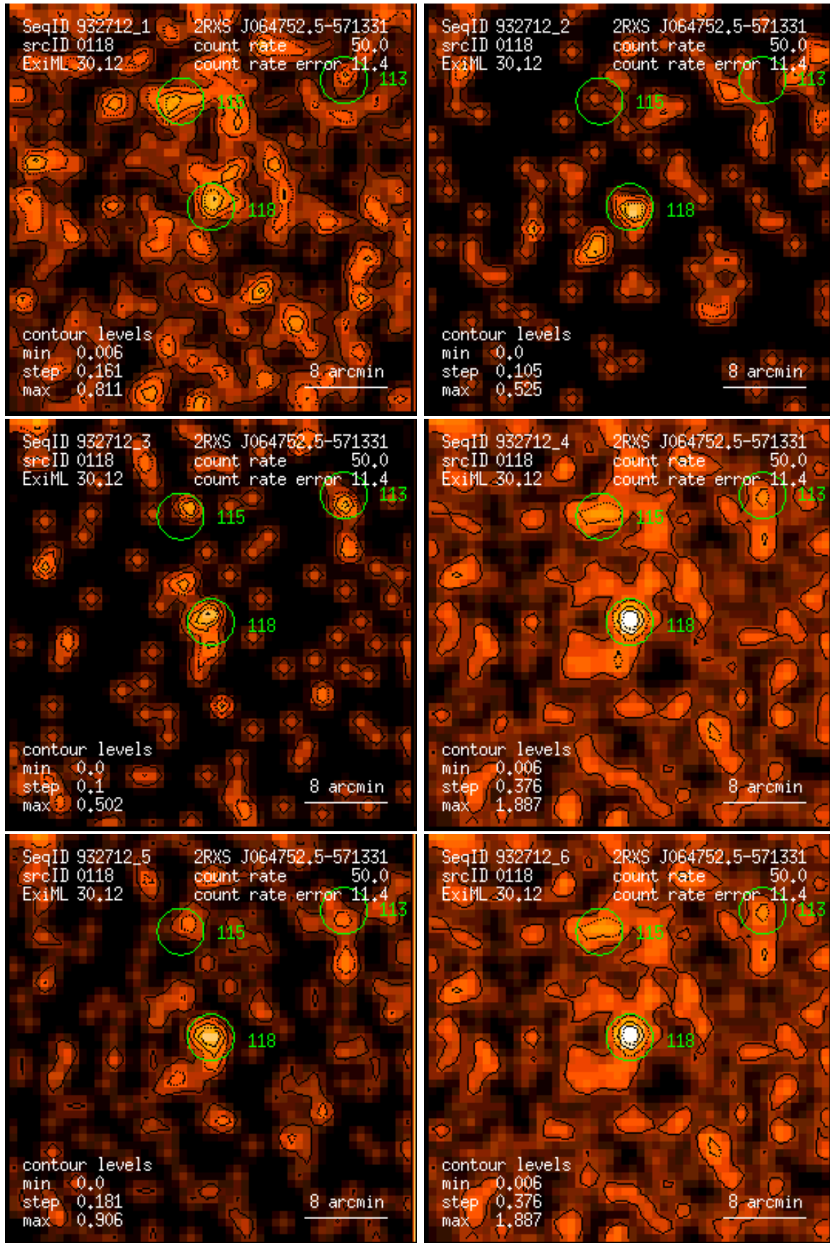
Figure 118: RASS 932712: detection 0118: band rate images, Gaussian filter: (1) PSPC channels 11 – 41, (2) 52 – 90, (3) 91 – 201, (4) 11 – 235, (5) 52 – 201, (6) 11 – 201. Broad band rates in counts/ks. Band rate contour levels in counts/ks/arcmin 2 .
