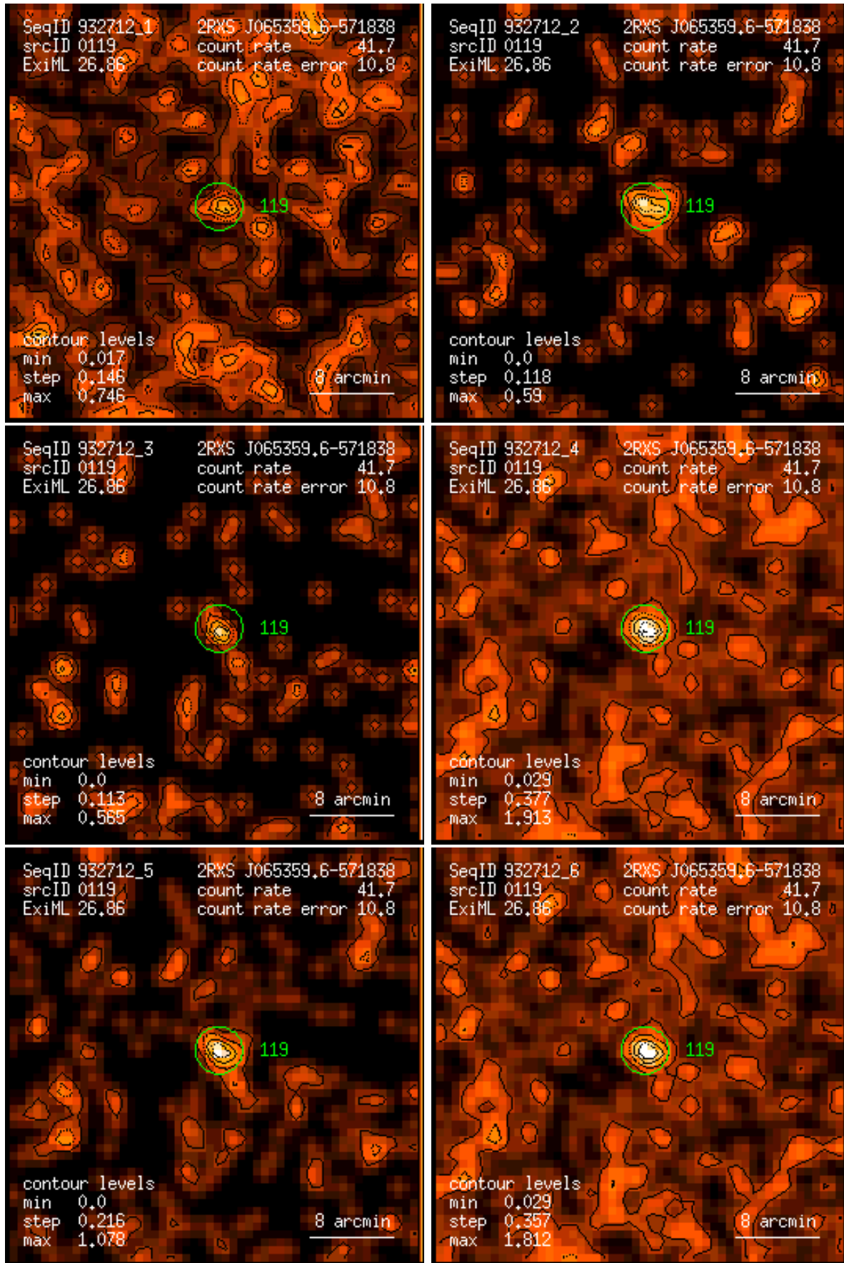
Figure 119: RASS 932712: detection 0119: band rate images, Gaussian filter: (1) PSPC channels 11 – 41, (2) 52 – 90, (3) 91 – 201, (4) 11 – 235, (5) 52 – 201, (6) 11 – 201. Broad band rates in counts/ks. Band rate contour levels in counts/ks/arcmin 2 .
