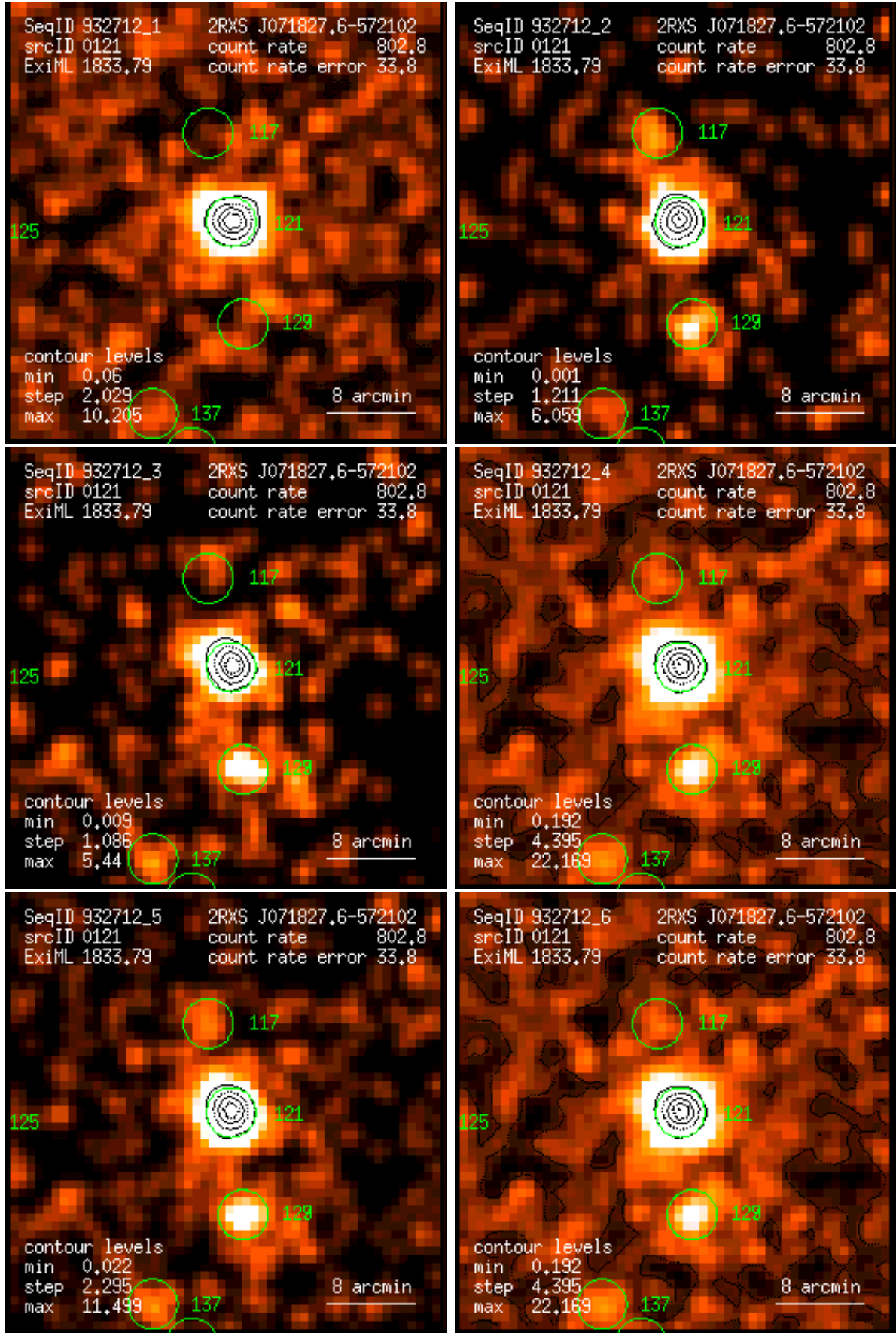
Figure 121: RASS 932712: detection 0121: band rate images, Gaussian filter: (1) PSPC channels 11 – 41, (2) 52 – 90, (3) 91 – 201, (4) 11 – 235, (5) 52 – 201, (6) 11 – 201. Broad band rates in counts/ks. Band rate contour levels in counts/ks/arcmin 2 .
