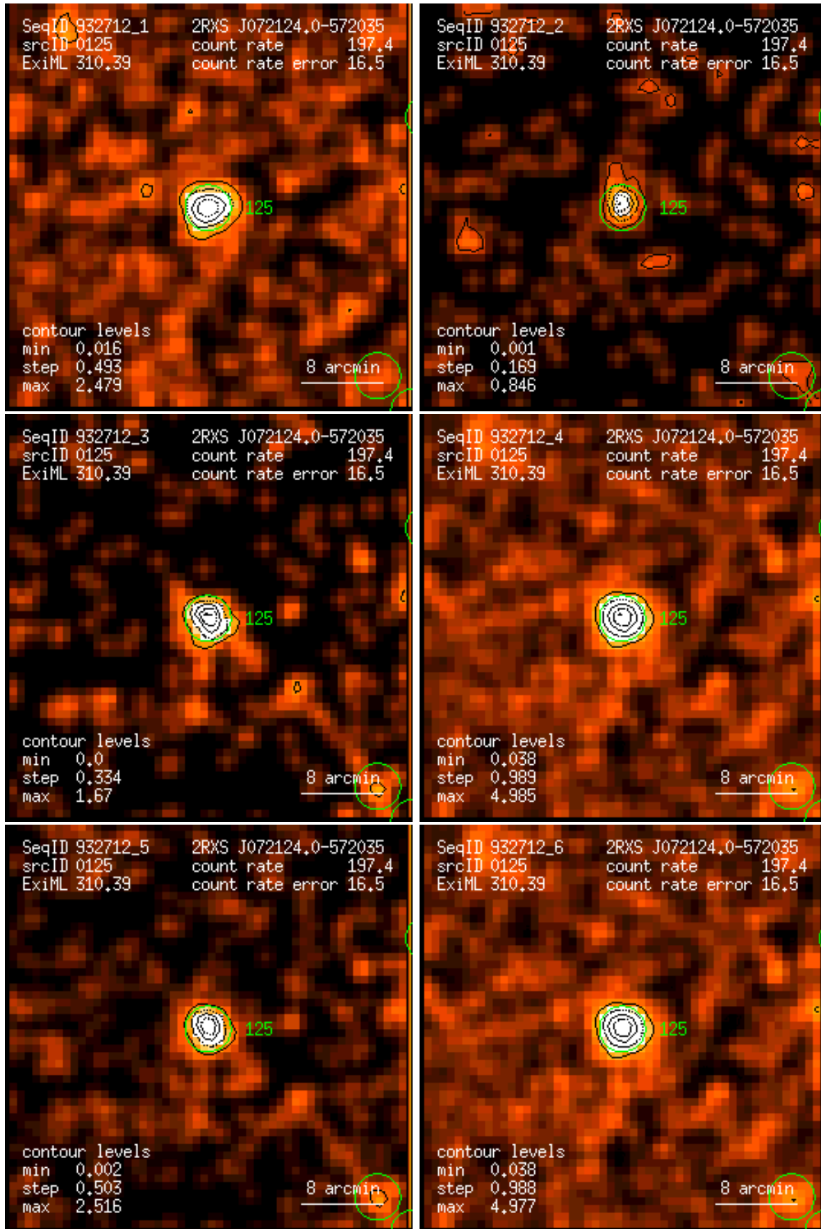
Figure 125: RASS 932712: detection 0125: band rate images, Gaussian filter: (1) PSPC channels 11 – 41, (2) 52 – 90, (3) 91 – 201, (4) 11 – 235, (5) 52 – 201, (6) 11 – 201. Broad band rates in counts/ks. Band rate contour levels in counts/ks/arcmin 2 .
