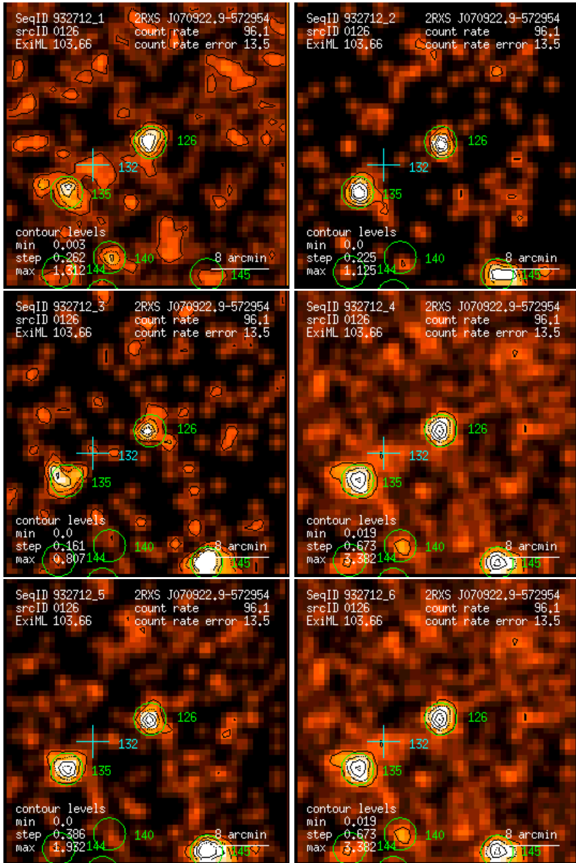
Figure 126: RASS 932712: detection 0126: band rate images, Gaussian filter: (1) PSPC channels 11 – 41, (2) 52 – 90, (3) 91 – 201, (4) 11 – 235, (5) 52 – 201, (6) 11 – 201. Broad band rates in counts/ks. Band rate contour levels in counts/ks/arcmin 2 .
