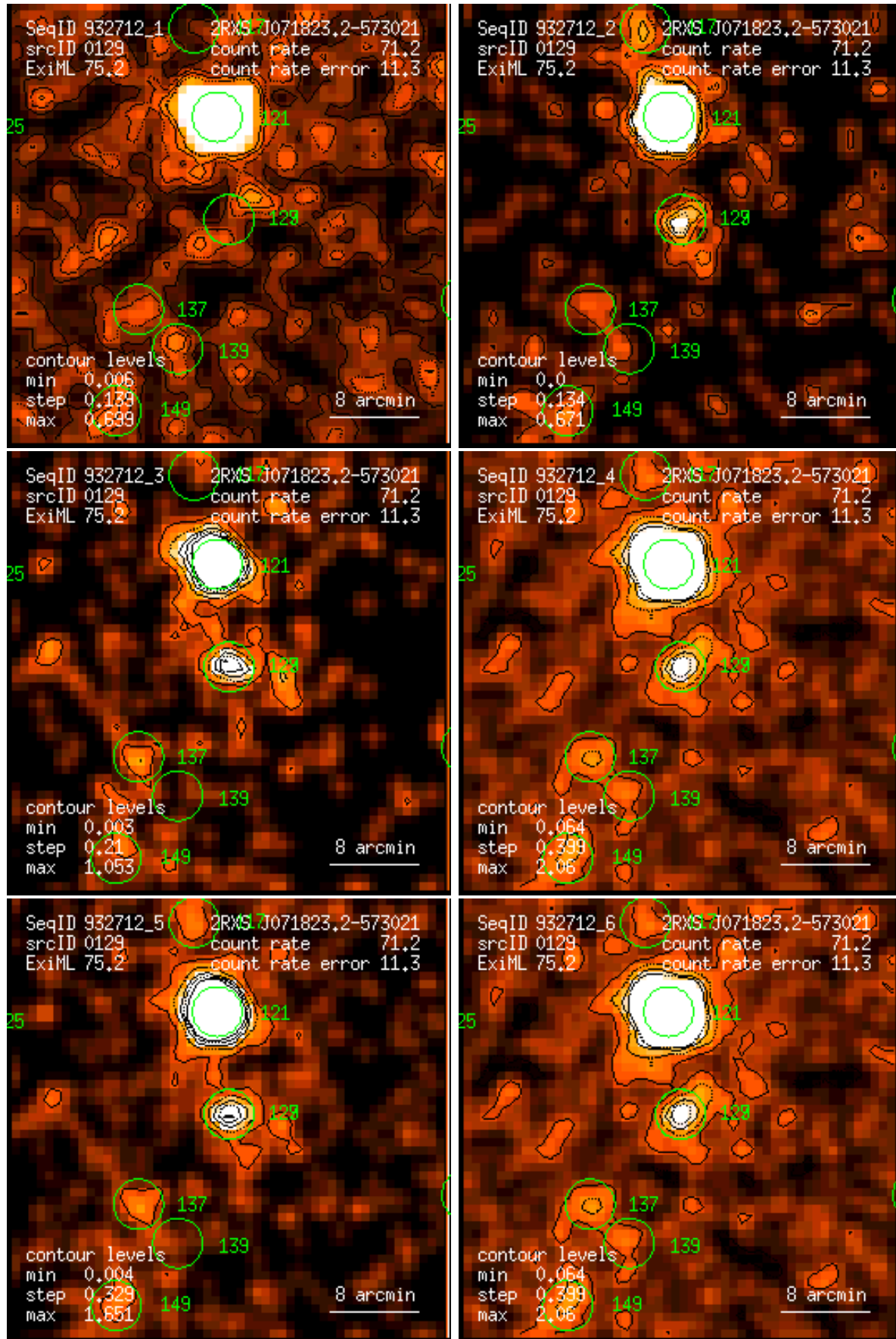
Figure 129: RASS 932712: detection 0129: band rate images, Gaussian filter: (1) PSPC channels 11 – 41, (2) 52 – 90, (3) 91 – 201, (4) 11 – 235, (5) 52 – 201, (6) 11 – 201. Broad band rates in counts/ks. Band rate contour levels in counts/ks/arcmin 2 .
