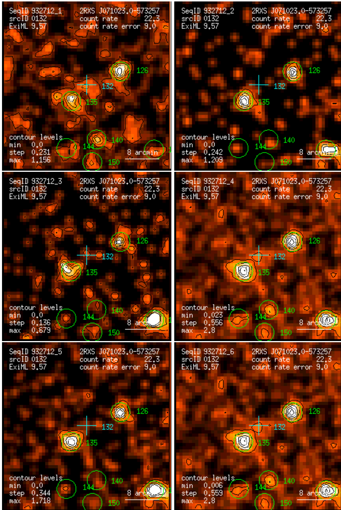
Figure 132: RASS 932712: detection 0132: band rate images, Gaussian filter: (1) PSPC channels 11 – 41, (2) 52 – 90, (3) 91 – 201, (4) 11 – 235, (5) 52 – 201, (6) 11 – 201. Broad band rates in counts/ks. Band rate contour levels in counts/ks/arcmin 2 .
