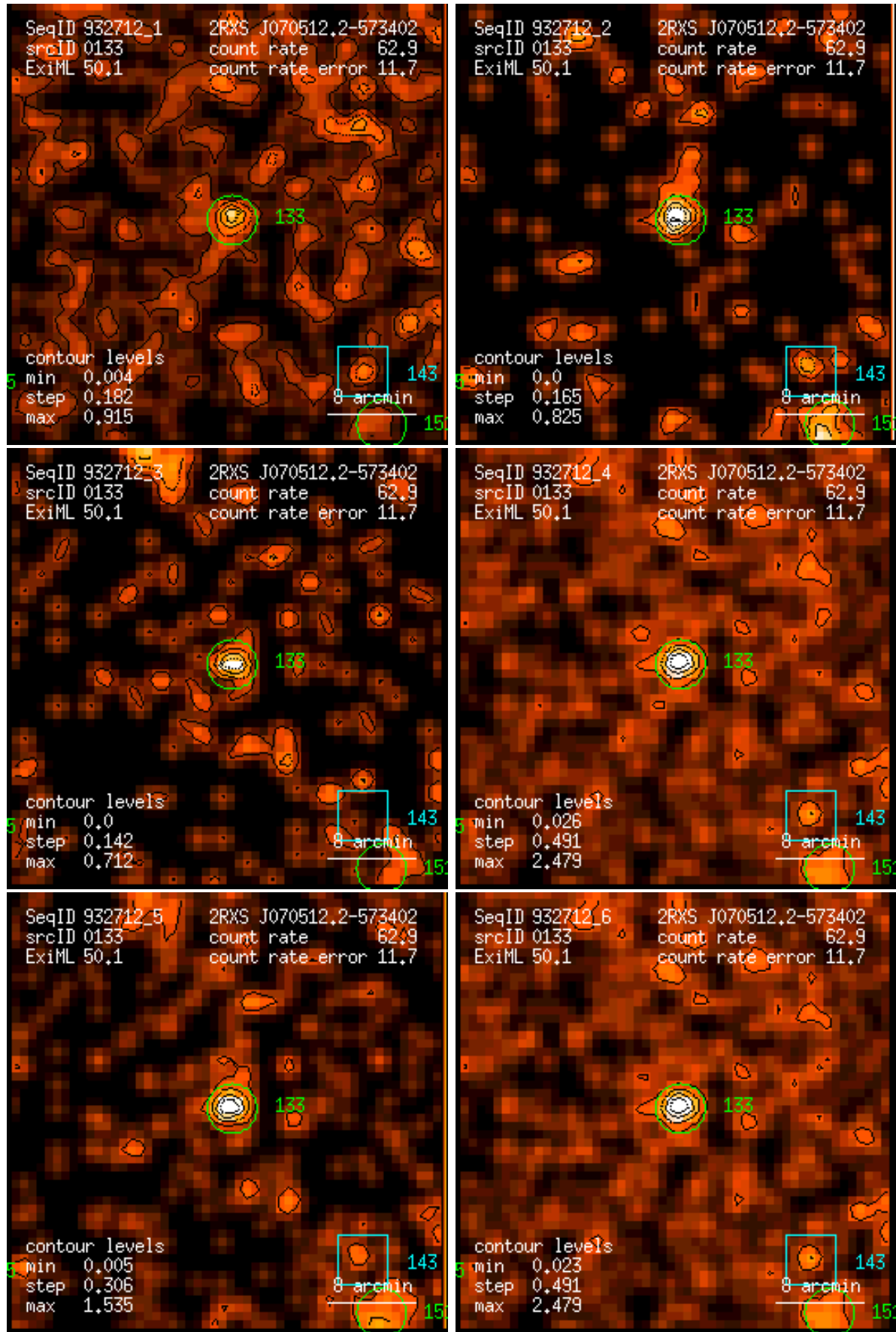
Figure 133: RASS 932712: detection 0133: band rate images, Gaussian filter: (1) PSPC channels 11 – 41, (2) 52 – 90, (3) 91 – 201, (4) 11 – 235, (5) 52 – 201, (6) 11 – 201. Broad band rates in counts/ks. Band rate contour levels in counts/ks/arcmin 2 .
