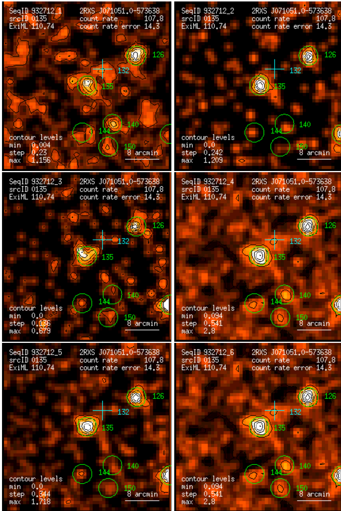
Figure 135: RASS 932712: detection 0135: band rate images, Gaussian filter: (1) PSPC channels 11 – 41, (2) 52 – 90, (3) 91 – 201, (4) 11 – 235, (5) 52 – 201, (6) 11 – 201. Broad band rates in counts/ks. Band rate contour levels in counts/ks/arcmin 2 .
