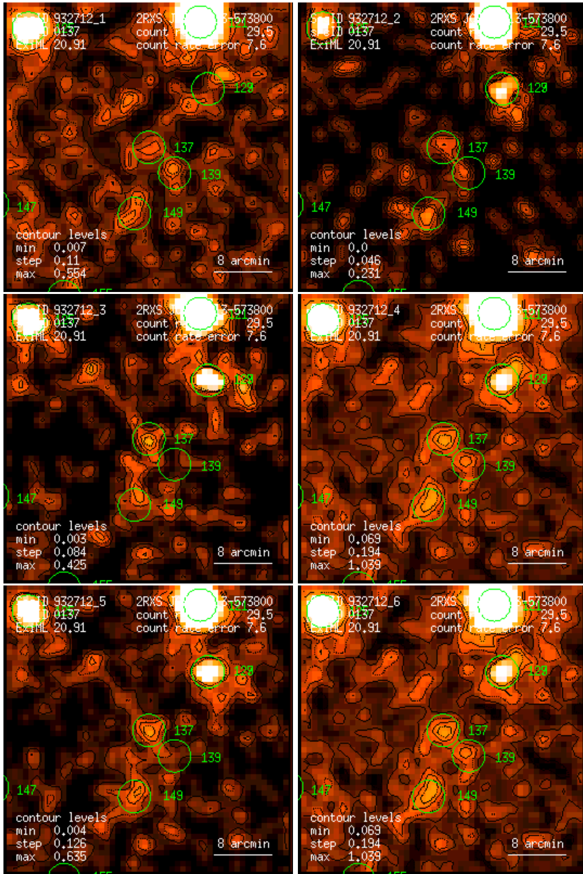
Figure 137: RASS 932712: detection 0137: band rate images, Gaussian filter: (1) PSPC channels 11 – 41, (2) 52 – 90, (3) 91 – 201, (4) 11 – 235, (5) 52 – 201, (6) 11 – 201. Broad band rates in counts/ks. Band rate contour levels in counts/ks/arcmin 2 .
