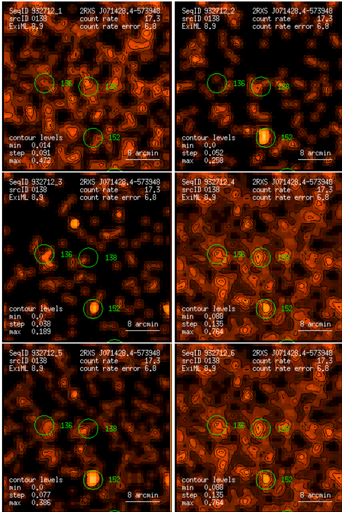
Figure 138: RASS 932712: detection 0138: band rate images, Gaussian filter: (1) PSPC channels 11 – 41, (2) 52 – 90, (3) 91 – 201, (4) 11 – 235, (5) 52 – 201, (6) 11 – 201. Broad band rates in counts/ks. Band rate contour levels in counts/ks/arcmin 2 .
