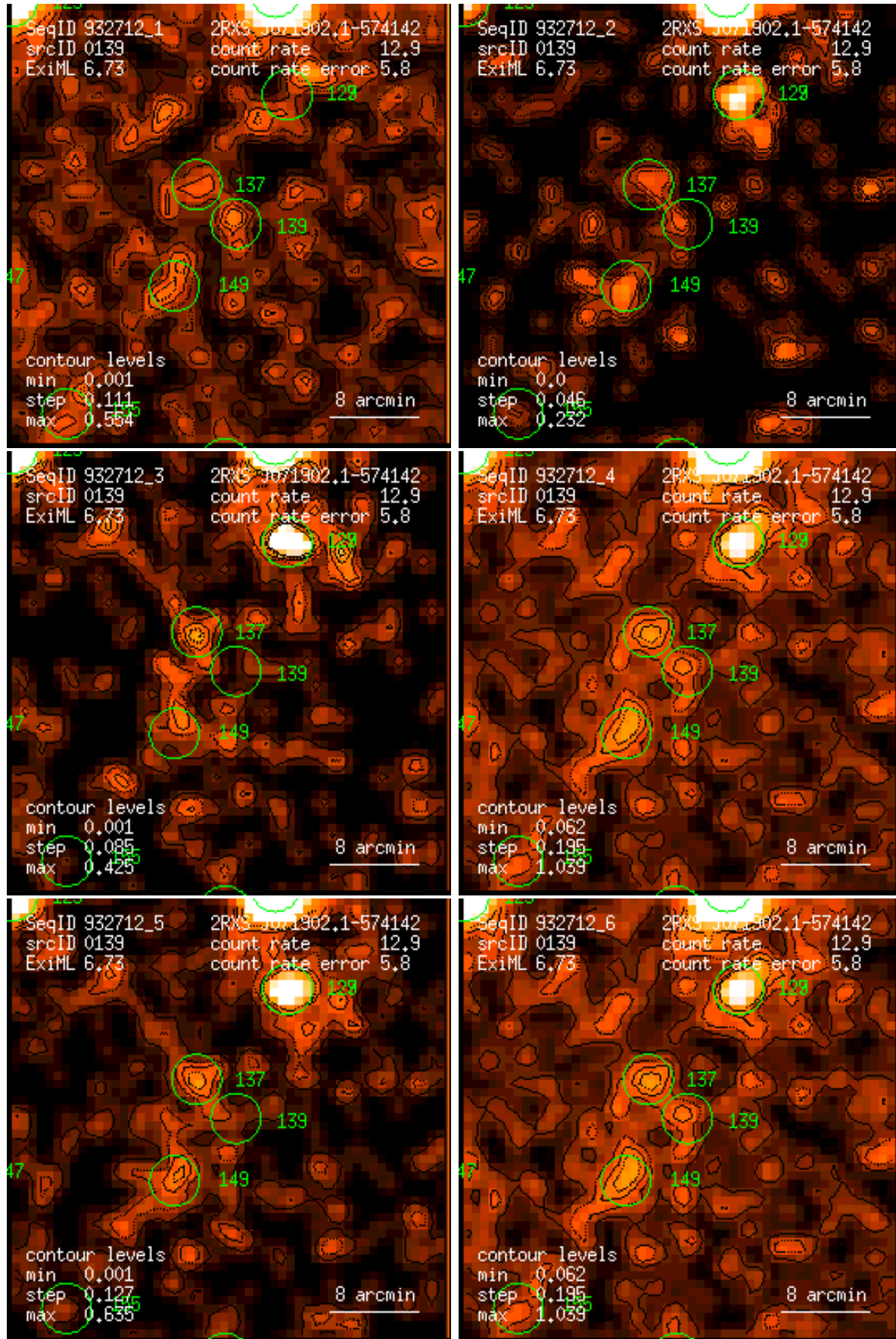
Figure 139: RASS 932712: detection 0139: band rate images, Gaussian filter: (1) PSPC channels 11 – 41, (2) 52 – 90, (3) 91 – 201, (4) 11 – 235, (5) 52 – 201, (6) 11 – 201. Broad band rates in counts/ks. Band rate contour levels in counts/ks/arcmin 2 .
