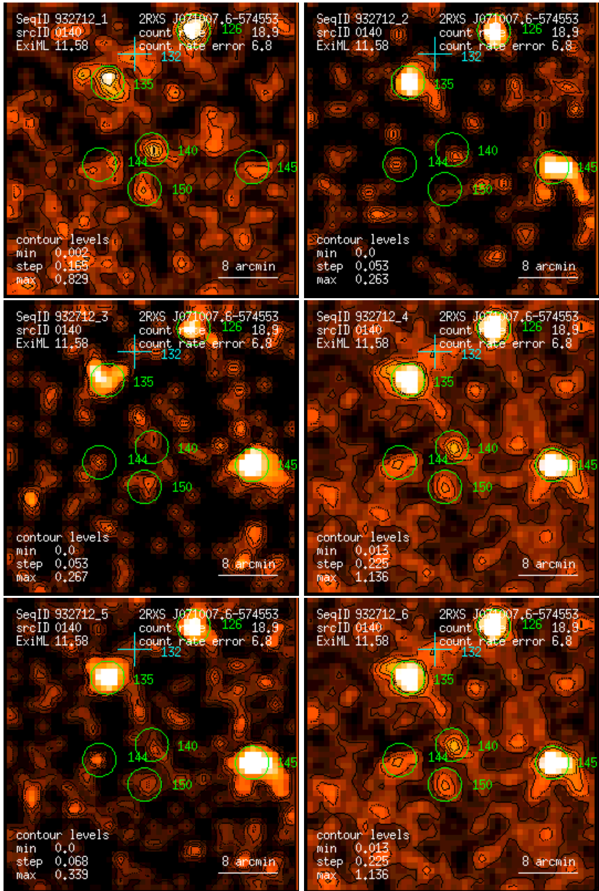
Figure 140: RASS 932712: detection 0140: band rate images, Gaussian filter: (1) PSPC channels 11 – 41, (2) 52 – 90, (3) 91 – 201, (4) 11 – 235, (5) 52 – 201, (6) 11 – 201. Broad band rates in counts/ks. Band rate contour levels in counts/ks/arcmin 2 .
