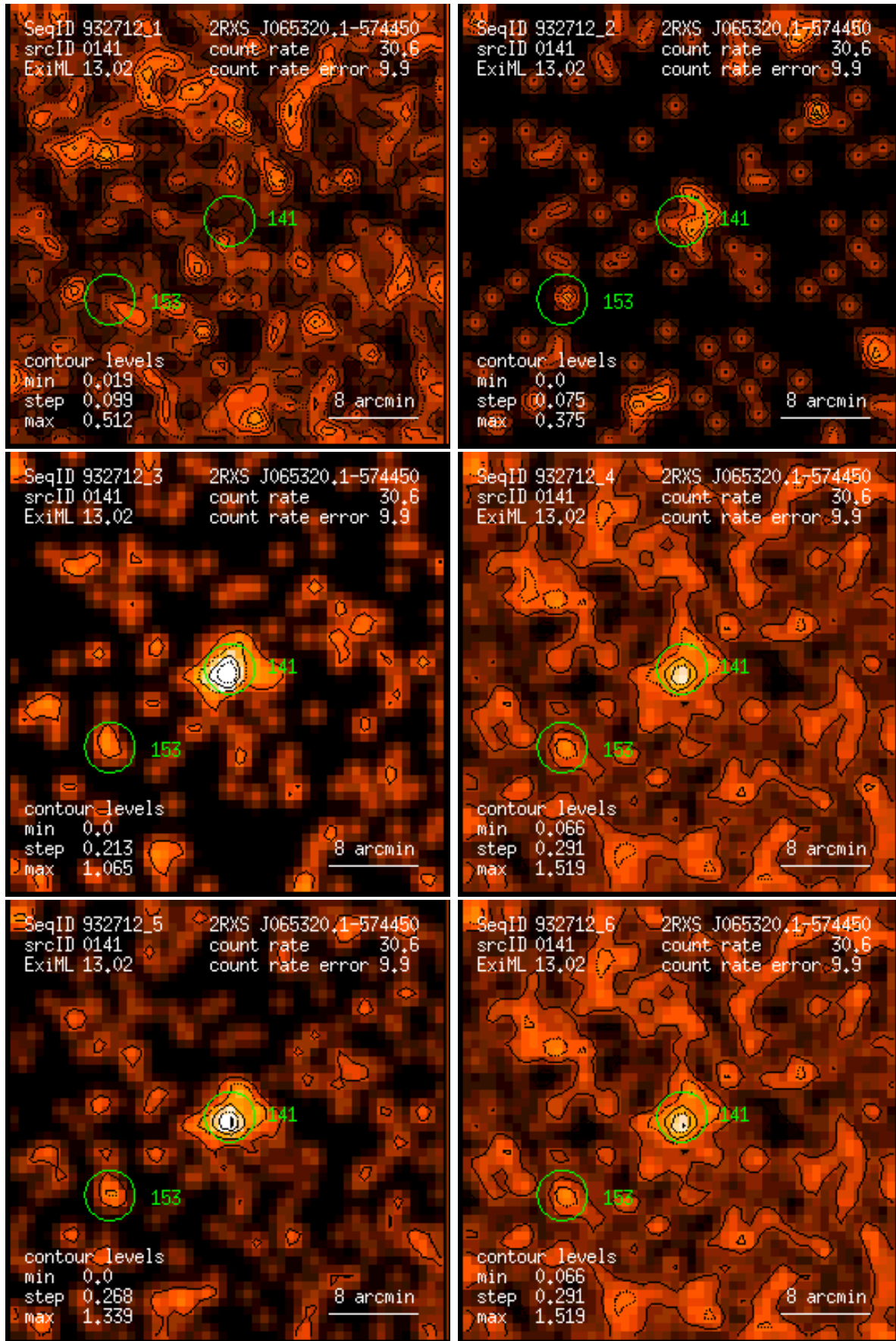
Figure 141: RASS 932712: detection 0141: band rate images, Gaussian filter: (1) PSPC channels 11 – 41, (2) 52 – 90, (3) 91 – 201, (4) 11 – 235, (5) 52 – 201, (6) 11 – 201. Broad band rates in counts/ks. Band rate contour levels in counts/ks/arcmin 2 .
