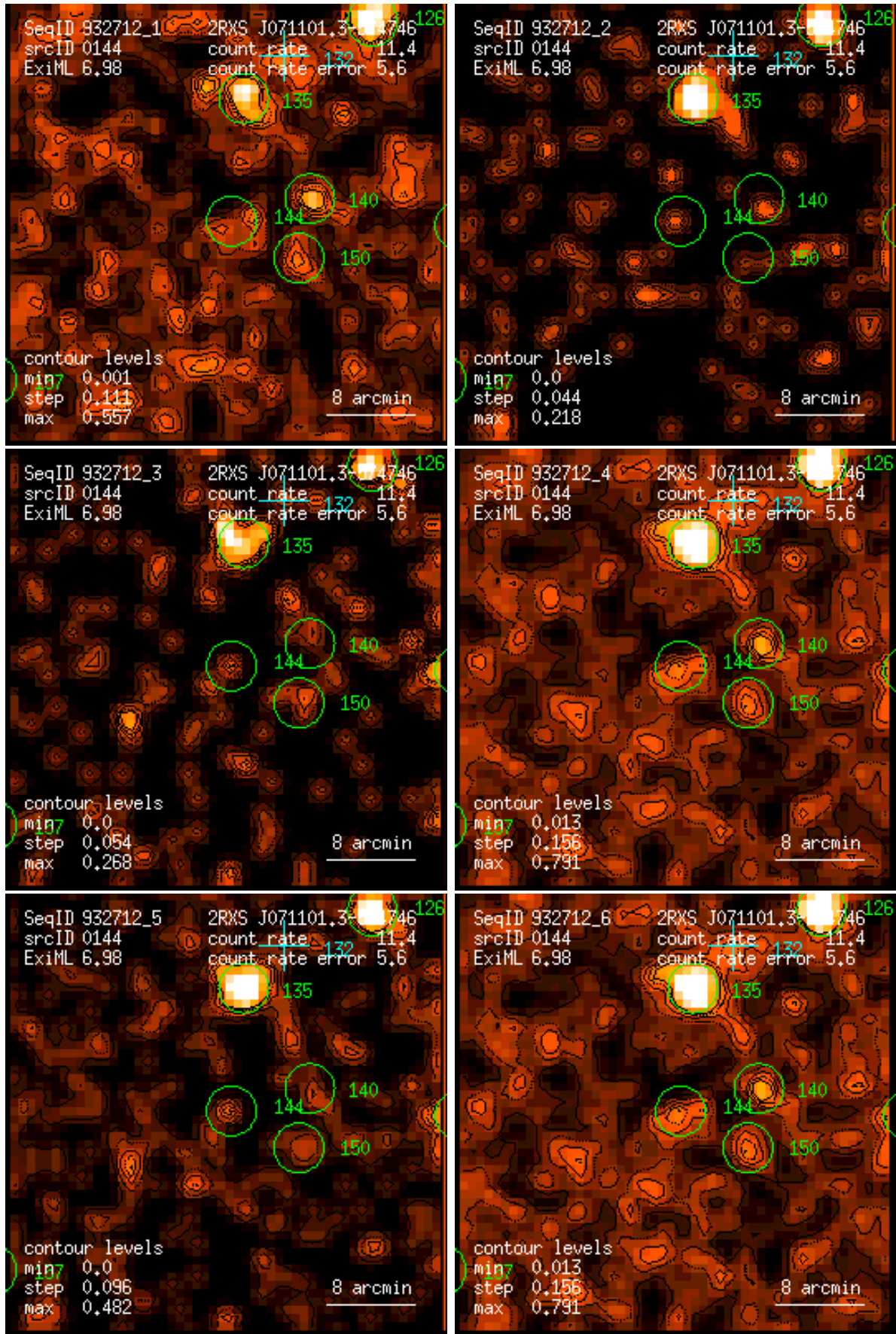
Figure 144: RASS 932712: detection 0144: band rate images, Gaussian filter: (1) PSPC channels 11 – 41, (2) 52 – 90, (3) 91 – 201, (4) 11 – 235, (5) 52 – 201, (6) 11 – 201. Broad band rates in counts/ks. Band rate contour levels in counts/ks/arcmin 2 .
