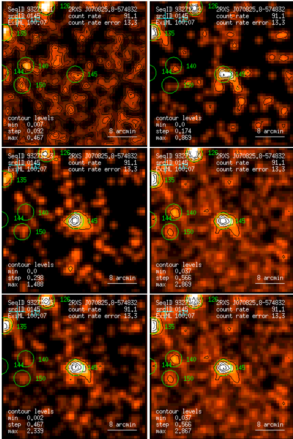
Figure 145: RASS 932712: detection 0145: band rate images, Gaussian filter: (1) PSPC channels 11 – 41, (2) 52 – 90, (3) 91 – 201, (4) 11 – 235, (5) 52 – 201, (6) 11 – 201. Broad band rates in counts/ks. Band rate contour levels in counts/ks/arcmin 2 .
