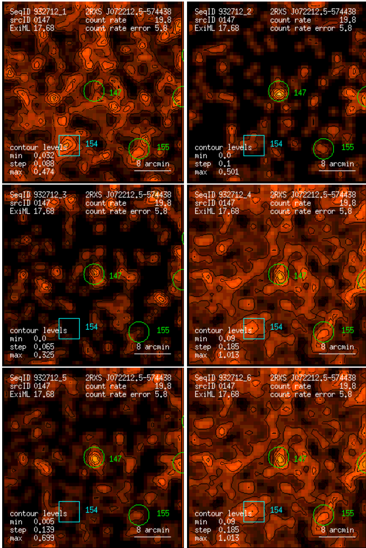
Figure 147: RASS 932712: detection 0147: band rate images, Gaussian filter: (1) PSPC channels 11 – 41, (2) 52 – 90, (3) 91 – 201, (4) 11 – 235, (5) 52 – 201, (6) 11 – 201. Broad band rates in counts/ks. Band rate contour levels in counts/ks/arcmin 2 .
