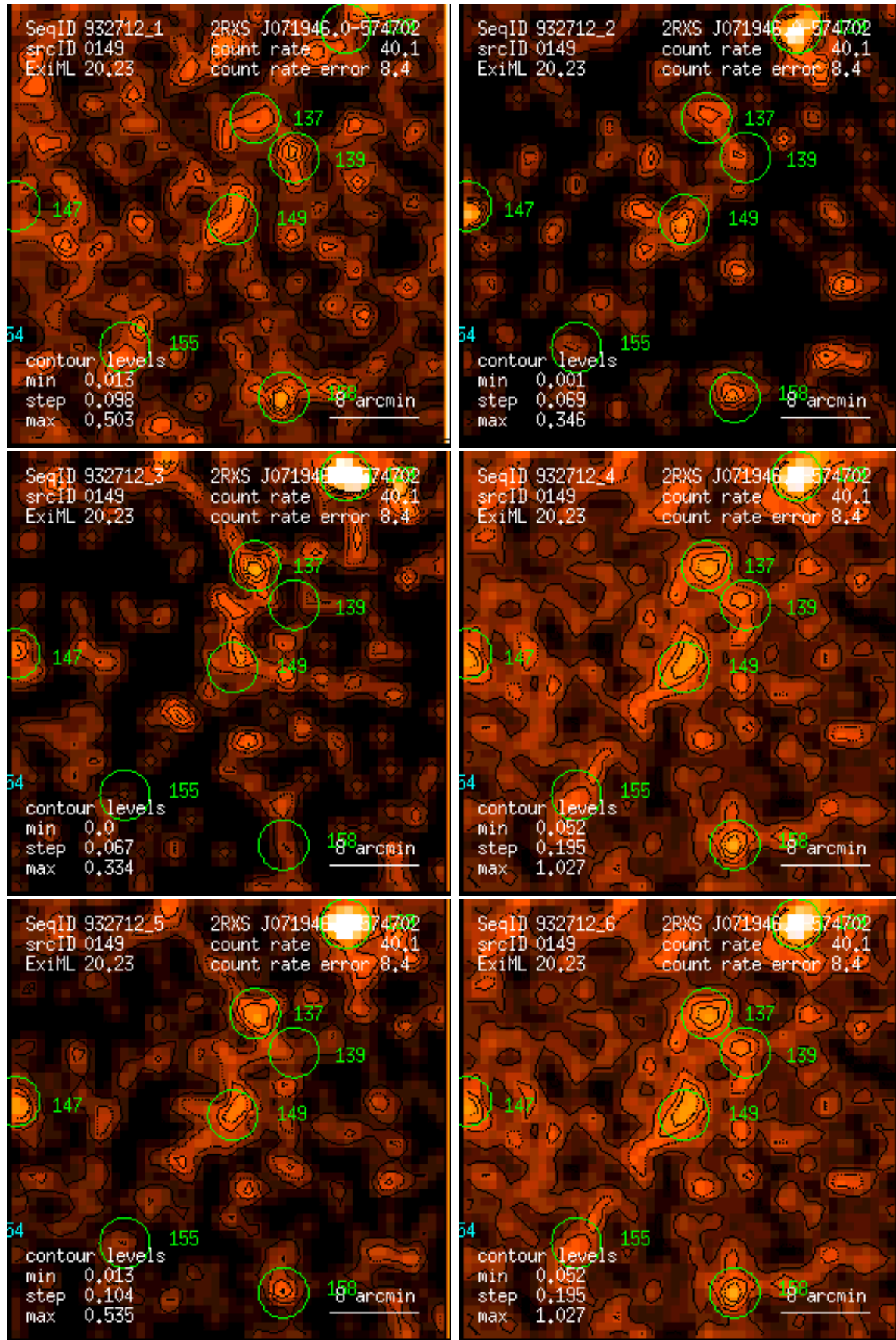
Figure 149: RASS 932712: detection 0149: band rate images, Gaussian filter: (1) PSPC channels 11 – 41, (2) 52 – 90, (3) 91 – 201, (4) 11 – 235, (5) 52 – 201, (6) 11 – 201. Broad band rates in counts/ks. Band rate contour levels in counts/ks/arcmin 2 .
