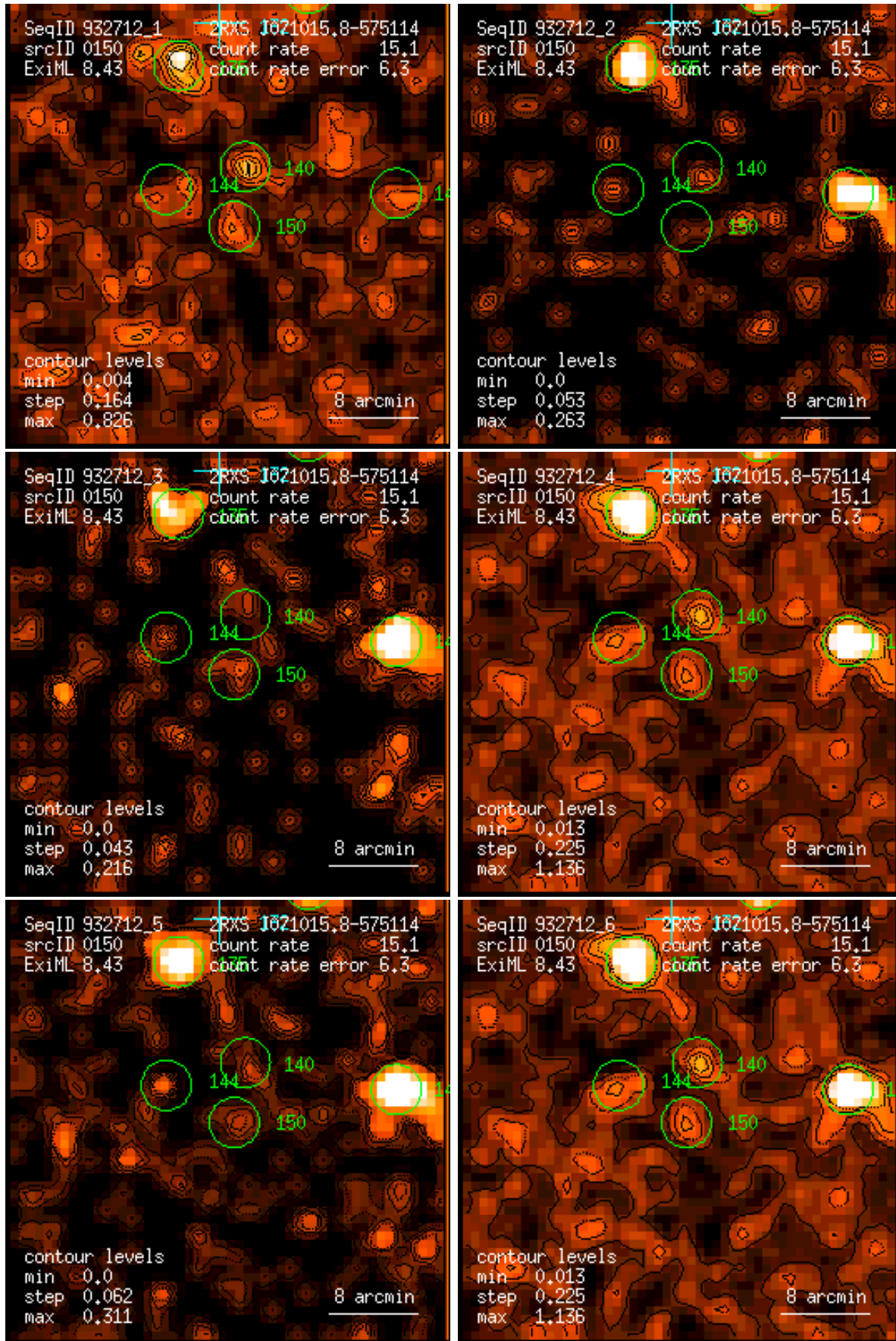
Figure 150: RASS 932712: detection 0150: band rate images, Gaussian filter: (1) PSPC channels 11 – 41, (2) 52 – 90, (3) 91 – 201, (4) 11 – 235, (5) 52 – 201, (6) 11 – 201. Broad band rates in counts/ks. Band rate contour levels in counts/ks/arcmin 2 .
