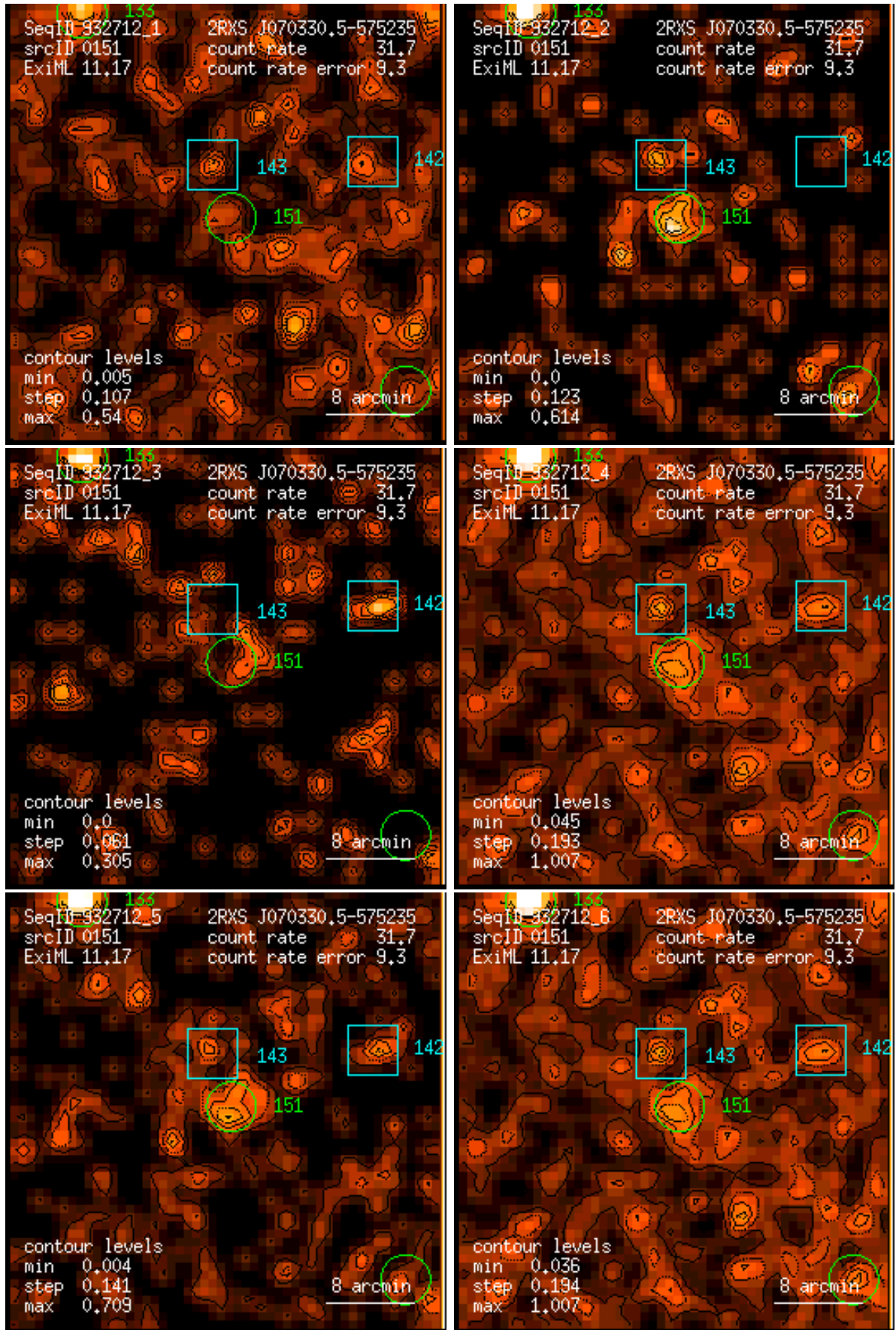
Figure 151: RASS 932712: detection 0151: band rate images, Gaussian filter: (1) PSPC channels 11 – 41, (2) 52 – 90, (3) 91 – 201, (4) 11 – 235, (5) 52 – 201, (6) 11 – 201. Broad band rates in counts/ks. Band rate contour levels in counts/ks/arcmin 2 .
