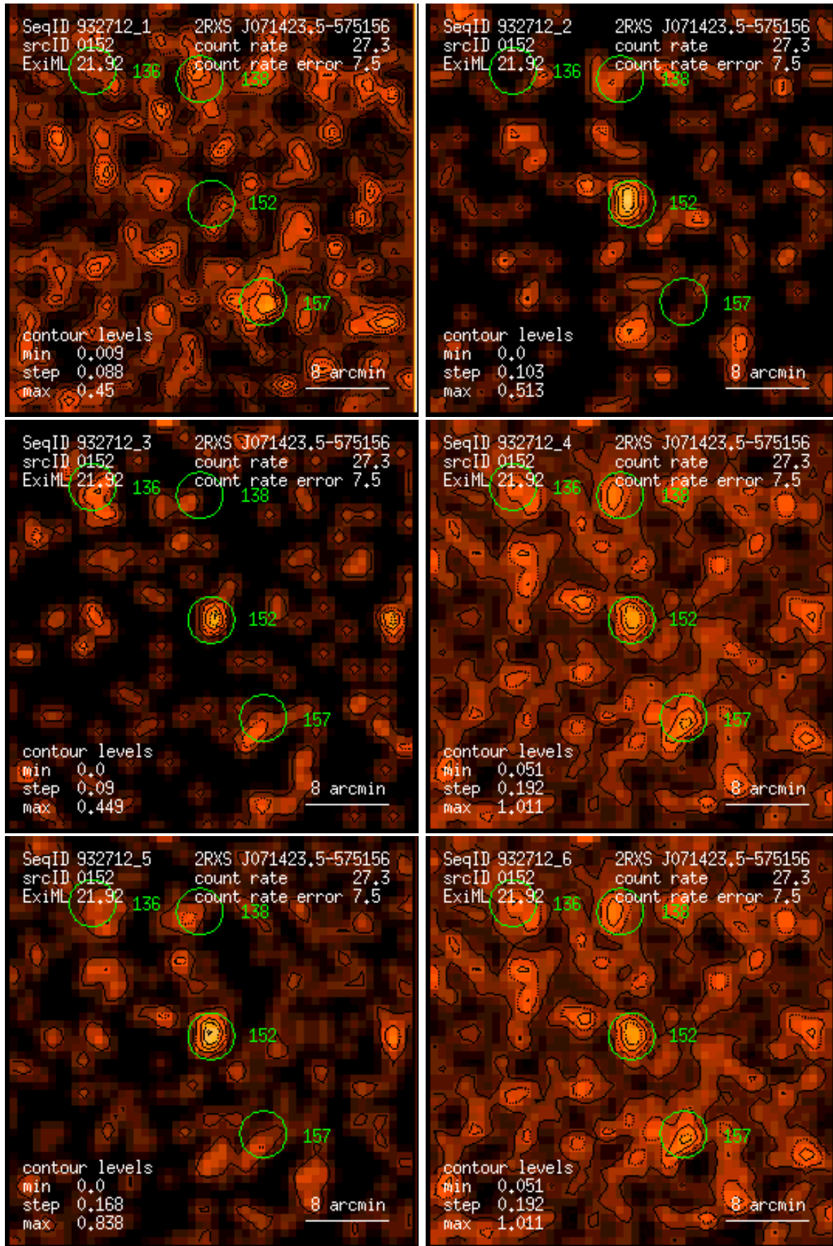
Figure 152: RASS 932712: detection 0152: band rate images, Gaussian filter: (1) PSPC channels 11 – 41, (2) 52 – 90, (3) 91 – 201, (4) 11 – 235, (5) 52 – 201, (6) 11 – 201. Broad band rates in counts/ks. Band rate contour levels in counts/ks/arcmin 2 .
