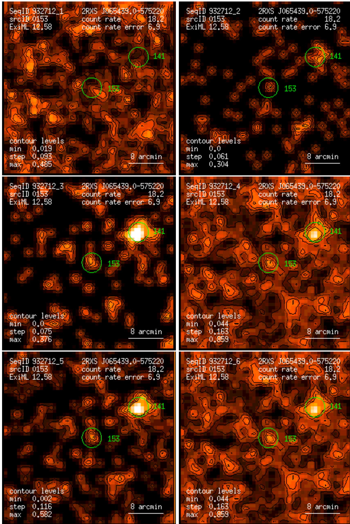
Figure 153: RASS 932712: detection 0153: band rate images, Gaussian filter: (1) PSPC channels 11 – 41, (2) 52 – 90, (3) 91 – 201, (4) 11 – 235, (5) 52 – 201, (6) 11 – 201. Broad band rates in counts/ks. Band rate contour levels in counts/ks/arcmin 2 .
