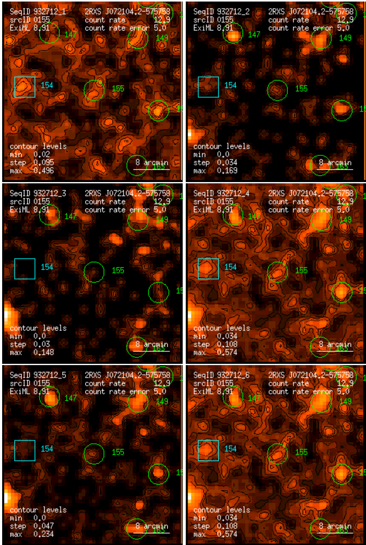
Figure 155: RASS 932712: detection 0155: band rate images, Gaussian filter: (1) PSPC channels 11 – 41, (2) 52 – 90, (3) 91 – 201, (4) 11 – 235, (5) 52 – 201, (6) 11 – 201. Broad band rates in counts/ks. Band rate contour levels in counts/ks/arcmin 2 .
