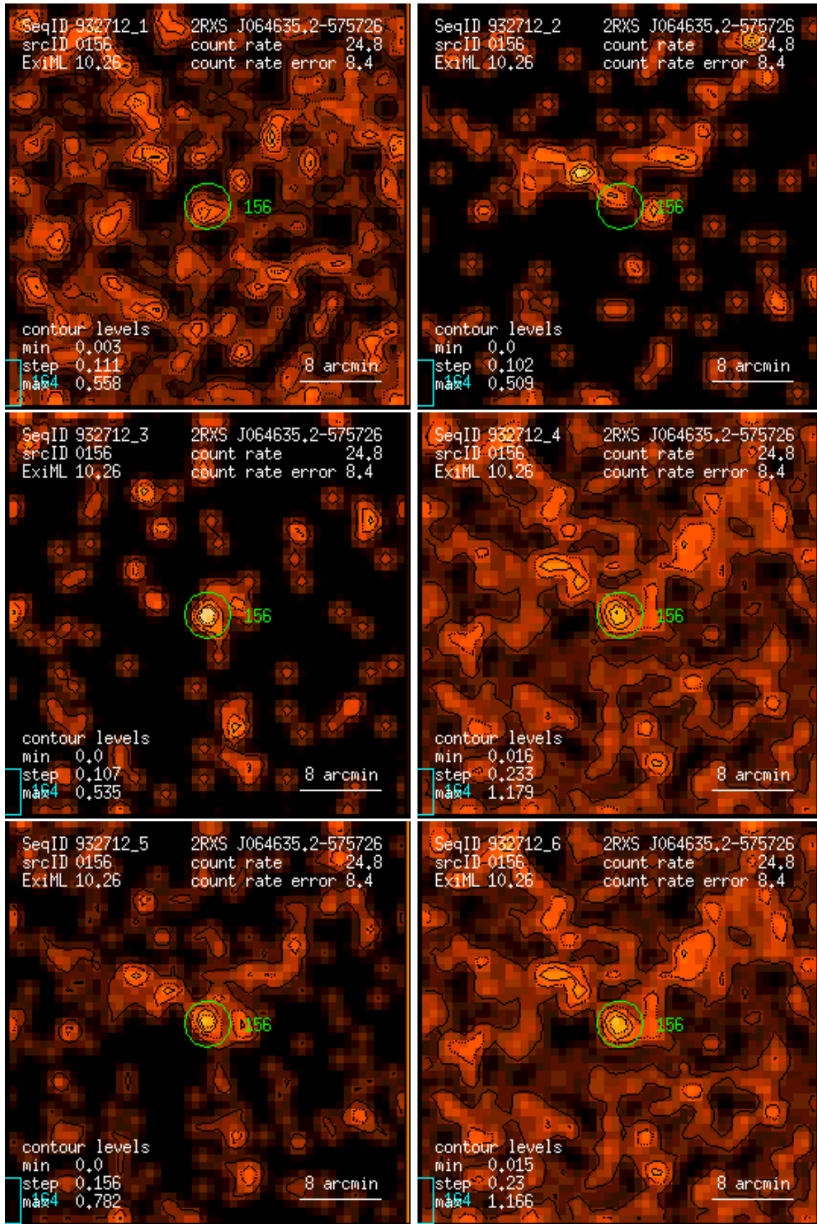
Figure 156: RASS 932712: detection 0156: band rate images, Gaussian filter: (1) PSPC channels 11 – 41, (2) 52 – 90, (3) 91 – 201, (4) 11 – 235, (5) 52 – 201, (6) 11 – 201. Broad band rates in counts/ks. Band rate contour levels in counts/ks/arcmin 2 .
