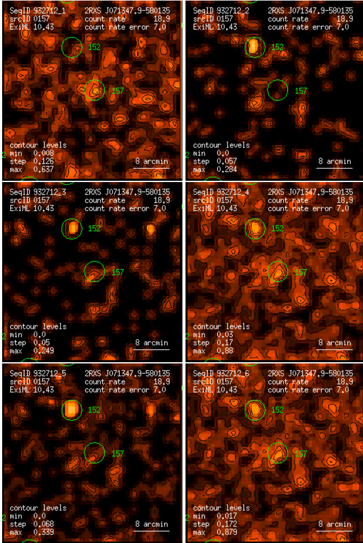
Figure 157: RASS 932712: detection 0157: band rate images, Gaussian filter: (1) PSPC channels 11 – 41, (2) 52 – 90, (3) 91 – 201, (4) 11 – 235, (5) 52 – 201, (6) 11 – 201. Broad band rates in counts/ks. Band rate contour levels in counts/ks/arcmin 2 .
